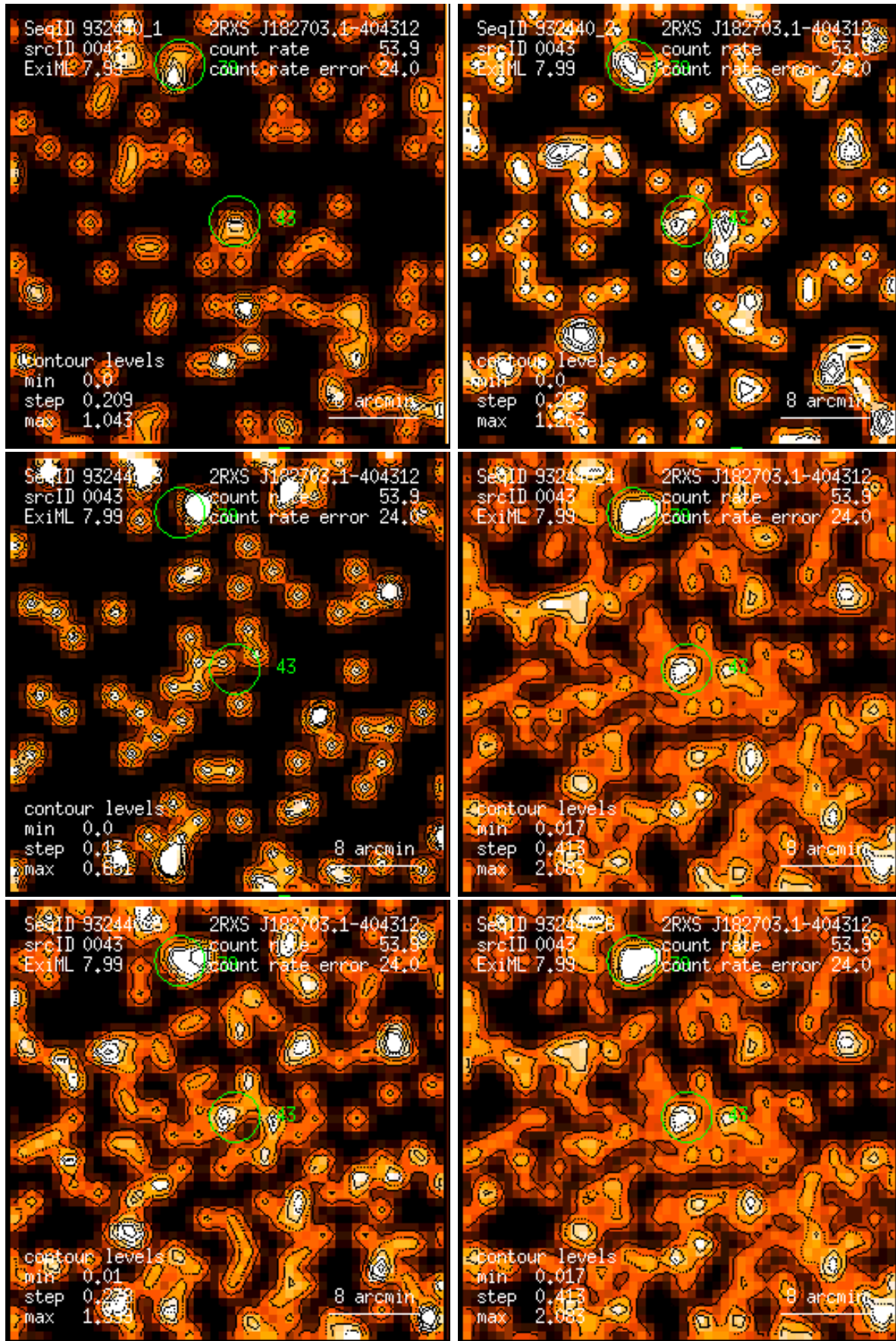
Figure 43: RASS 932440: detection 0043: band rate images, Gaussian filter: (1) PSPC channels 11 – 41, (2) 52 – 90, (3) 91 – 201, (4) 11 – 235, (5) 52 – 201, (6) 11 – 201. Broad band rates in counts/ks. Band rate contour levels in counts/ks/arcmin 2 .
