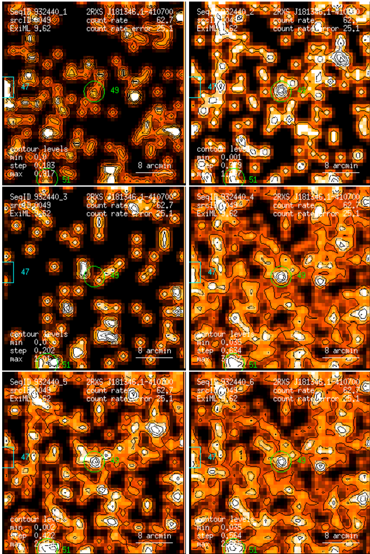
Figure 49: RASS 932440: detection 0049: band rate images, Gaussian filter: (1) PSPC channels 11 – 41, (2) 52 – 90, (3) 91 – 201, (4) 11 – 235, (5) 52 – 201, (6) 11 – 201. Broad band rates in counts/ks. Band rate contour levels in counts/ks/arcmin 2 .
