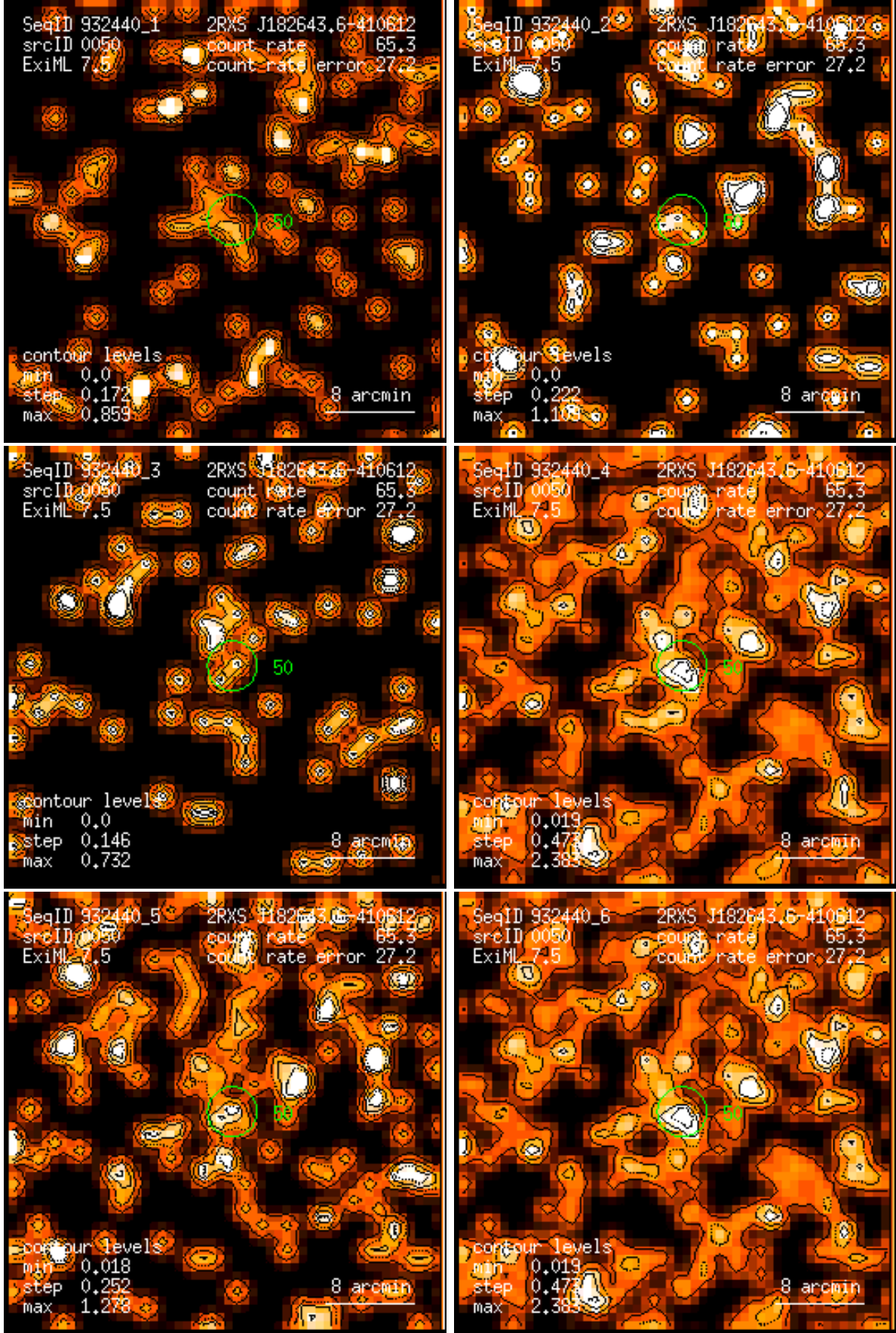
Figure 50: RASS 932440: detection 0050: band rate images, Gaussian filter: (1) PSPC channels 11 – 41, (2) 52 – 90, (3) 91 – 201, (4) 11 – 235, (5) 52 – 201, (6) 11 – 201. Broad band rates in counts/ks. Band rate contour levels in counts/ks/arcmin 2 .
