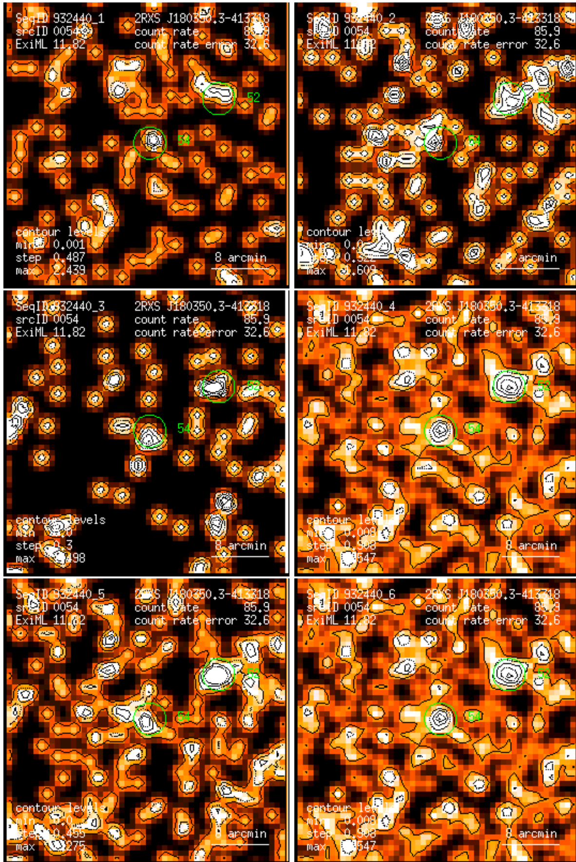
Figure 54: RASS 932440: detection 0054: band rate images, Gaussian filter: (1) PSPC channels 11 – 41, (2) 52 – 90, (3) 91 – 201, (4) 11 – 235, (5) 52 – 201, (6) 11 – 201. Broad band rates in counts/ks. Band rate contour levels in counts/ks/arcmin 2 .
