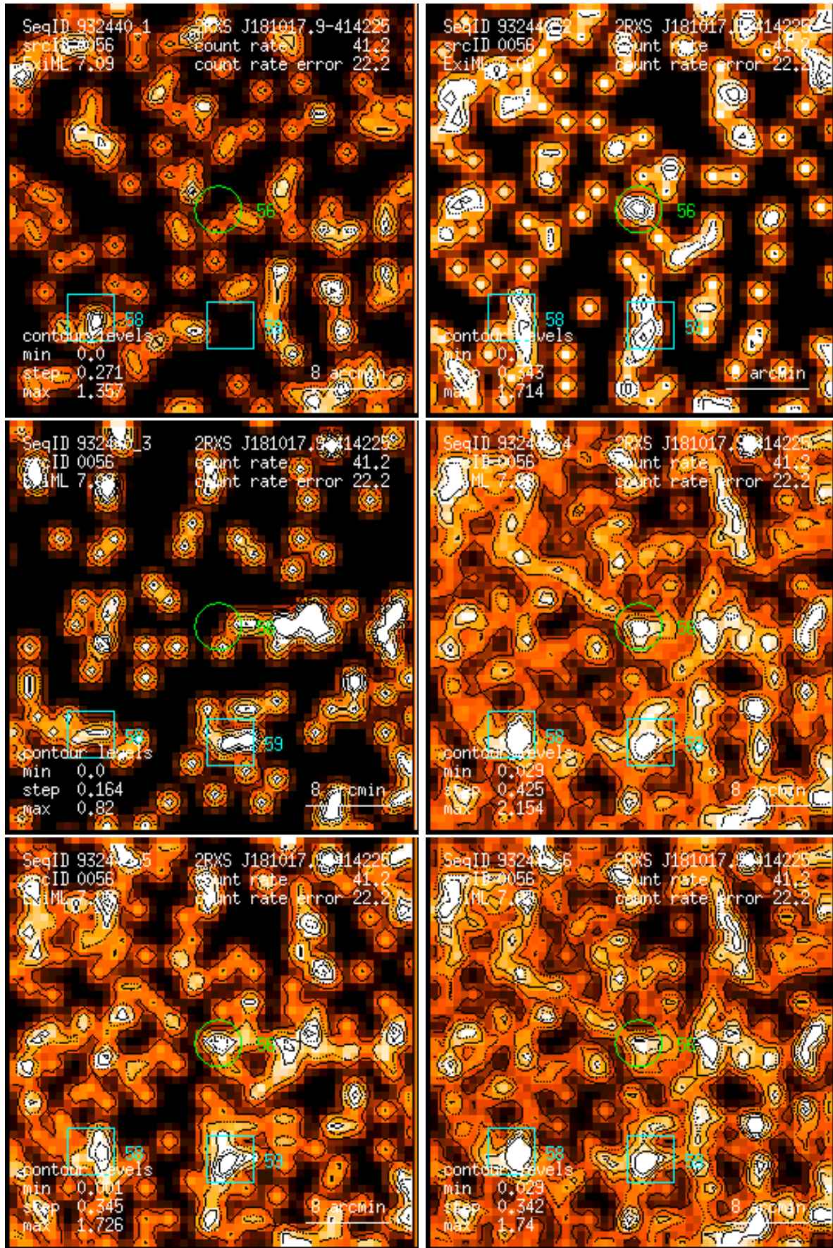
Figure 56: RASS 932440: detection 0056: band rate images, Gaussian filter: (1) PSPC channels 11 – 41, (2) 52 – 90, (3) 91 – 201, (4) 11 – 235, (5) 52 – 201, (6) 11 – 201. Broad band rates in counts/ks. Band rate contour levels in counts/ks/arcmin 2 .
