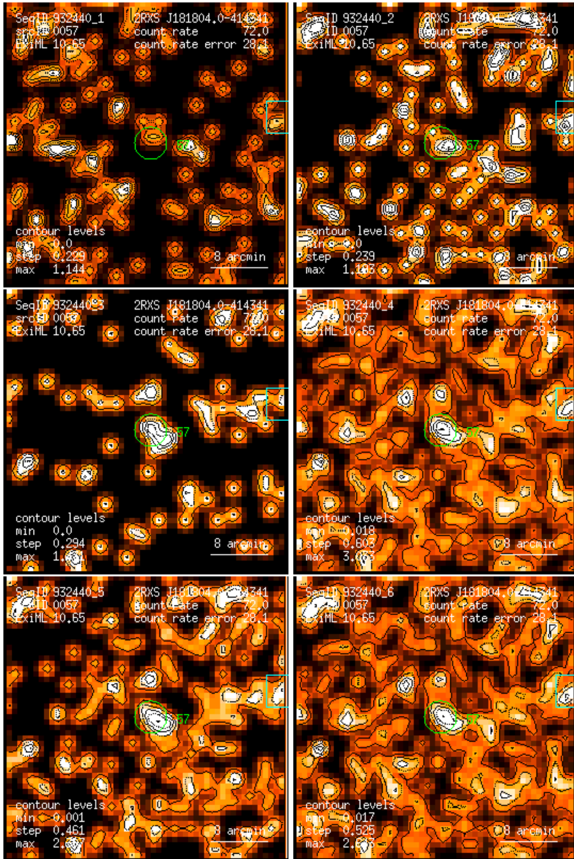
Figure 57: RASS 932440: detection 0057: band rate images, Gaussian filter: (1) PSPC channels 11 – 41, (2) 52 – 90, (3) 91 – 201, (4) 11 – 235, (5) 52 – 201, (6) 11 – 201. Broad band rates in counts/ks. Band rate contour levels in counts/ks/arcmin 2 .
