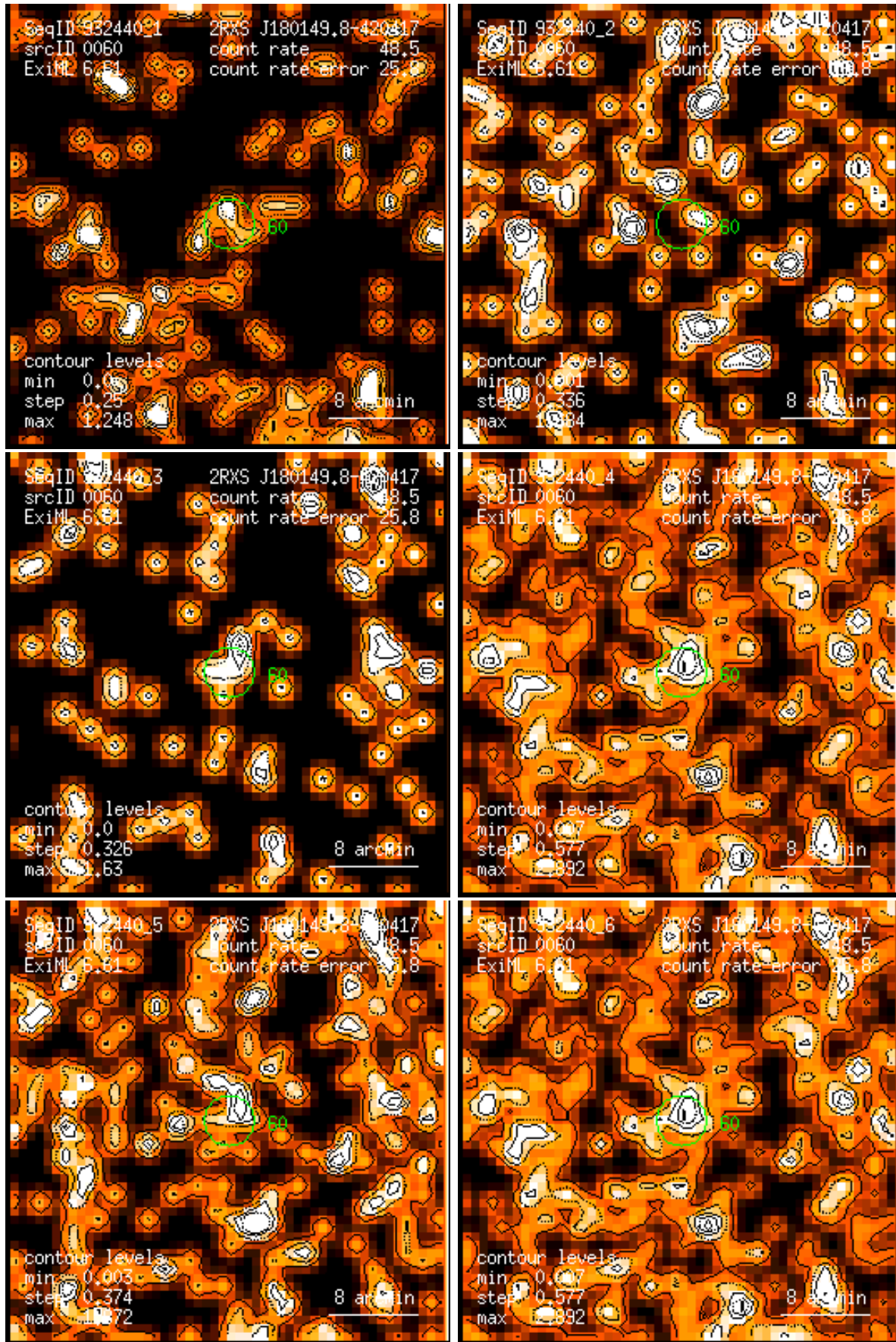
Figure 60: RASS 932440: detection 0060: band rate images, Gaussian filter: (1) PSPC channels 11 – 41, (2) 52 – 90, (3) 91 – 201, (4) 11 – 235, (5) 52 – 201, (6) 11 – 201. Broad band rates in counts/ks. Band rate contour levels in counts/ks/arcmin 2 .
