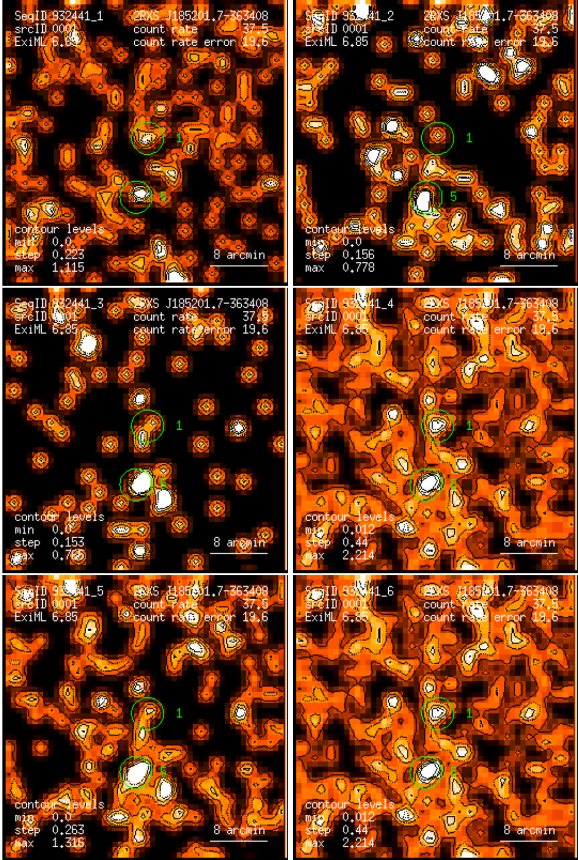
Figure 1: RASS 932441: detection 0001: band rate images, Gaussian filter: (1) PSPC channels 11 – 41, (2) 52 – 90, (3) 91 – 201, (4) 11 – 235, (5) 52 – 201, (6) 11 – 201. Broad band rates in counts/ks. Band rate contour levels in counts/ks/arcmin 2 .
