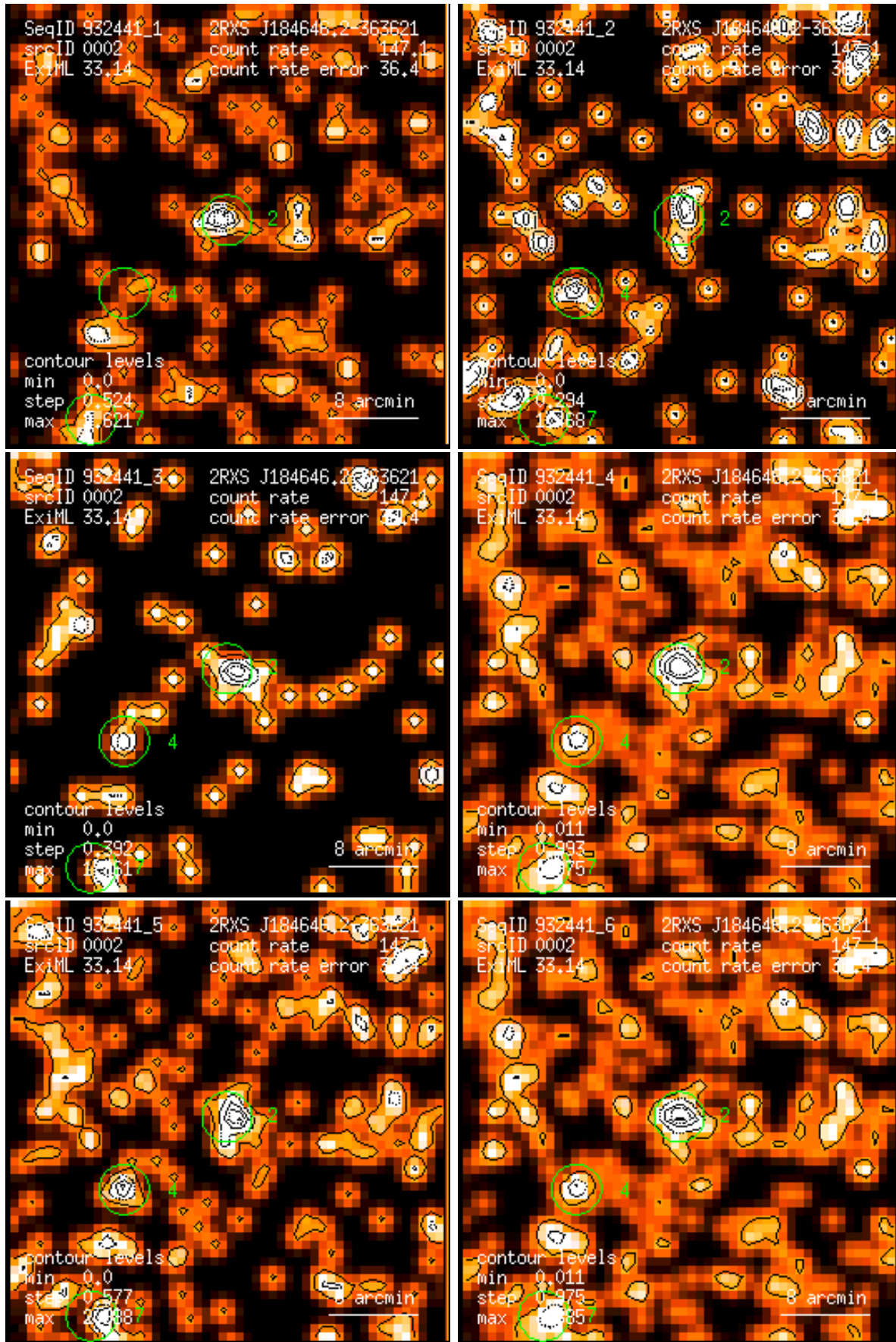
Figure 2: RASS 932441: detection 0002: band rate images, Gaussian filter: (1) PSPC channels 11 – 41, (2) 52 – 90, (3) 91 – 201, (4) 11 – 235, (5) 52 – 201, (6) 11 – 201. Broad band rates in counts/ks. Band rate contour levels in counts/ks/arcmin 2 .
