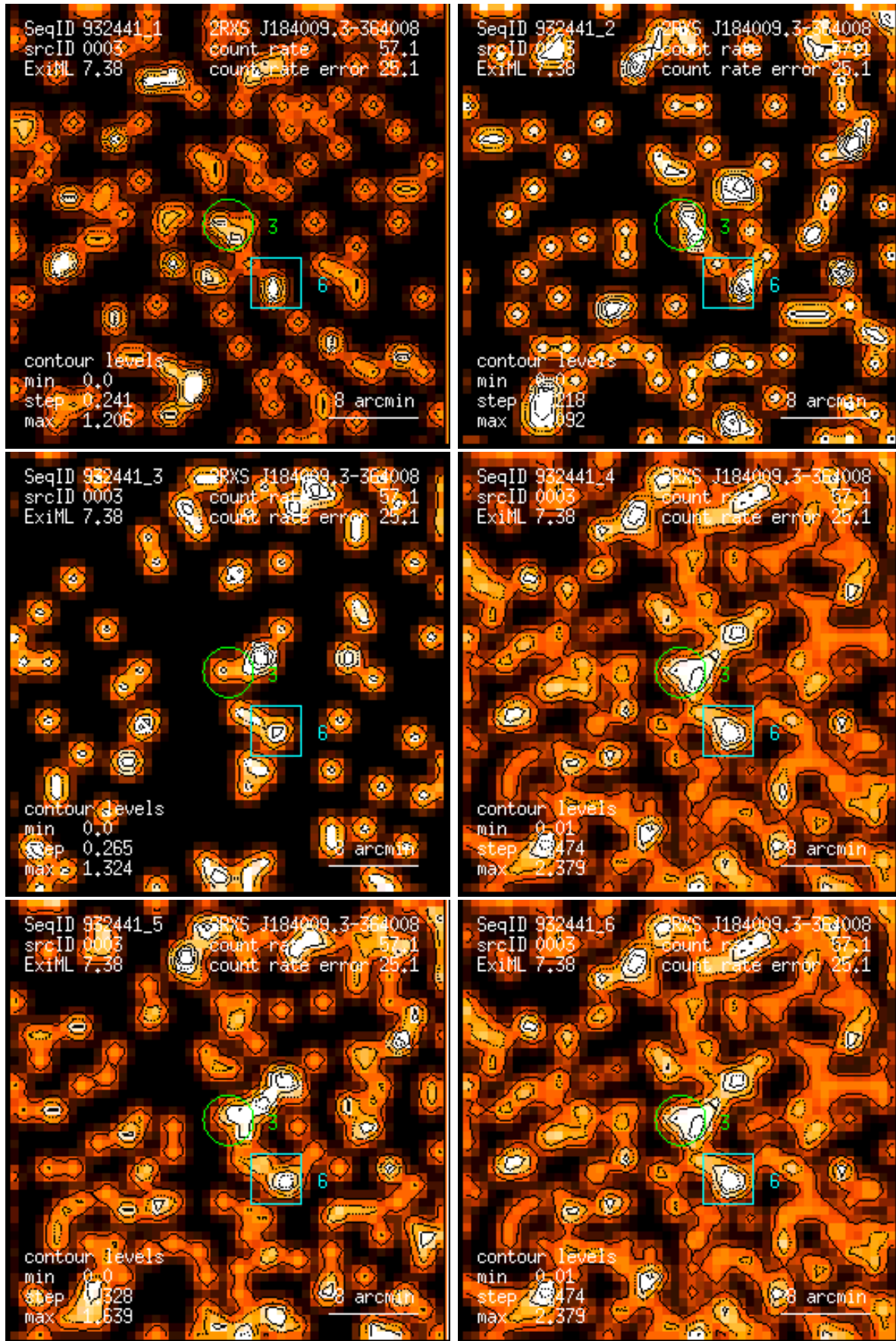
Figure 3: RASS 932441: detection 0003: band rate images, Gaussian filter: (1) PSPC channels 11 – 41, (2) 52 – 90, (3) 91 – 201, (4) 11 – 235, (5) 52 – 201, (6) 11 – 201. Broad band rates in counts/ks. Band rate contour levels in counts/ks/arcmin 2 .
