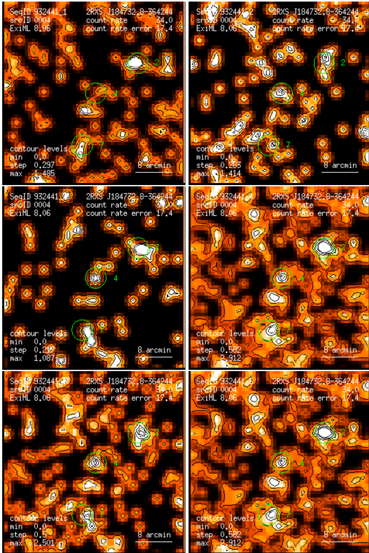
Figure 4: RASS 932441: detection 0004: band rate images, Gaussian filter: (1) PSPC channels 11 – 41, (2) 52 – 90, (3) 91 – 201, (4) 11 – 235, (5) 52 – 201, (6) 11 – 201. Broad band rates in counts/ks. Band rate contour levels in counts/ks/arcmin 2 .
