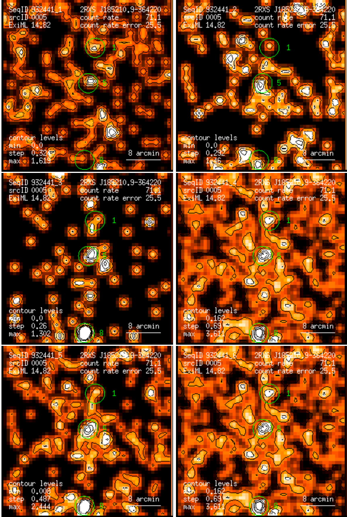
Figure 5: RASS 932441: detection 0005: band rate images, Gaussian filter: (1) PSPC channels 11 – 41, (2) 52 – 90, (3) 91 – 201, (4) 11 – 235, (5) 52 – 201, (6) 11 – 201. Broad band rates in counts/ks. Band rate contour levels in counts/ks/arcmin 2 .
