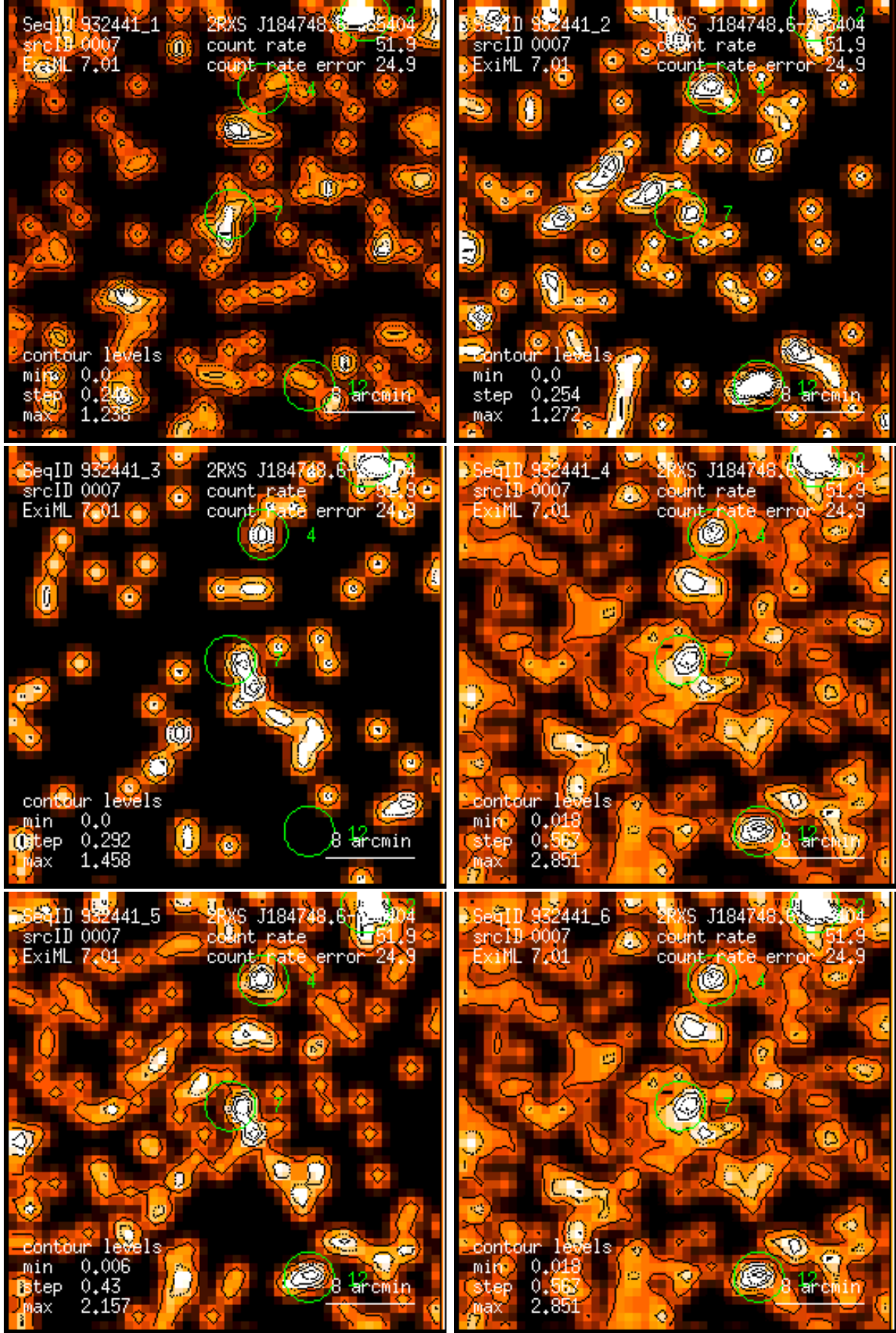
Figure 7: RASS 932441: detection 0007: band rate images, Gaussian filter: (1) PSPC channels 11 – 41, (2) 52 – 90, (3) 91 – 201, (4) 11 – 235, (5) 52 – 201, (6) 11 – 201. Broad band rates in counts/ks. Band rate contour levels in counts/ks/arcmin 2 .
