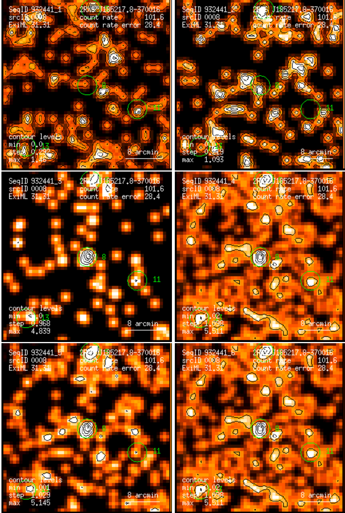
Figure 8: RASS 932441: detection 0008: band rate images, Gaussian filter: (1) PSPC channels 11 – 41, (2) 52 – 90, (3) 91 – 201, (4) 11 – 235, (5) 52 – 201, (6) 11 – 201. Broad band rates in counts/ks. Band rate contour levels in counts/ks/arcmin 2 .
