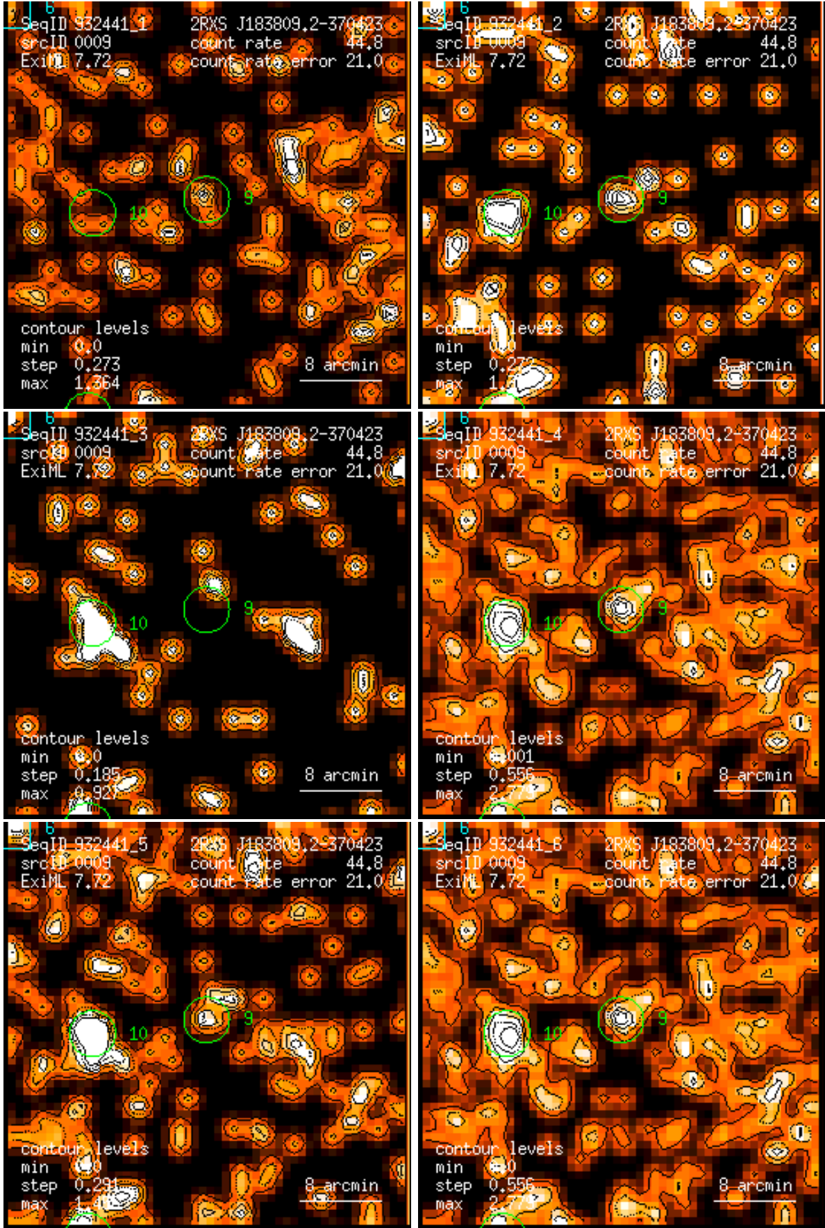
Figure 9: RASS 932441: detection 0009: band rate images, Gaussian filter: (1) PSPC channels 11 – 41, (2) 52 – 90, (3) 91 – 201, (4) 11 – 235, (5) 52 – 201, (6) 11 – 201. Broad band rates in counts/ks. Band rate contour levels in counts/ks/arcmin 2 .
