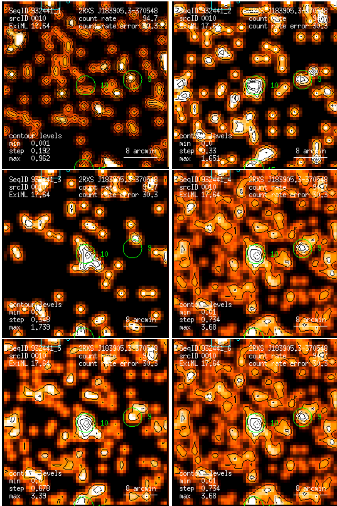
Figure 10: RASS 932441: detection 0010: band rate images, Gaussian filter: (1) PSPC channels 11 – 41, (2) 52 – 90, (3) 91 – 201, (4) 11 – 235, (5) 52 – 201, (6) 11 – 201. Broad band rates in counts/ks. Band rate contour levels in counts/ks/arcmin 2 .
