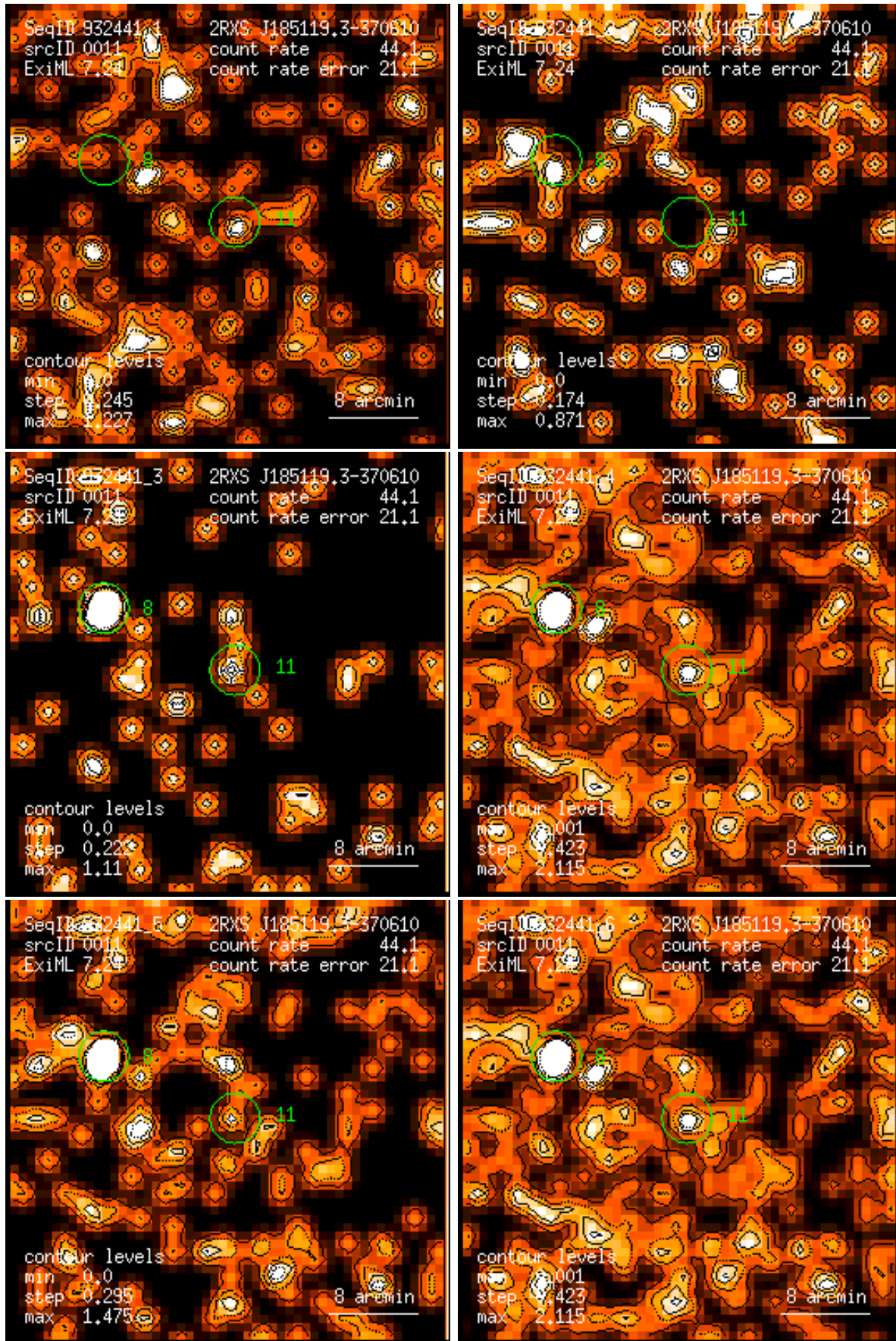
Figure 11: RASS 932441: detection 0011: band rate images, Gaussian filter: (1) PSPC channels 11 – 41, (2) 52 – 90, (3) 91 – 201, (4) 11 – 235, (5) 52 – 201, (6) 11 – 201. Broad band rates in counts/ks. Band rate contour levels in counts/ks/arcmin 2 .
