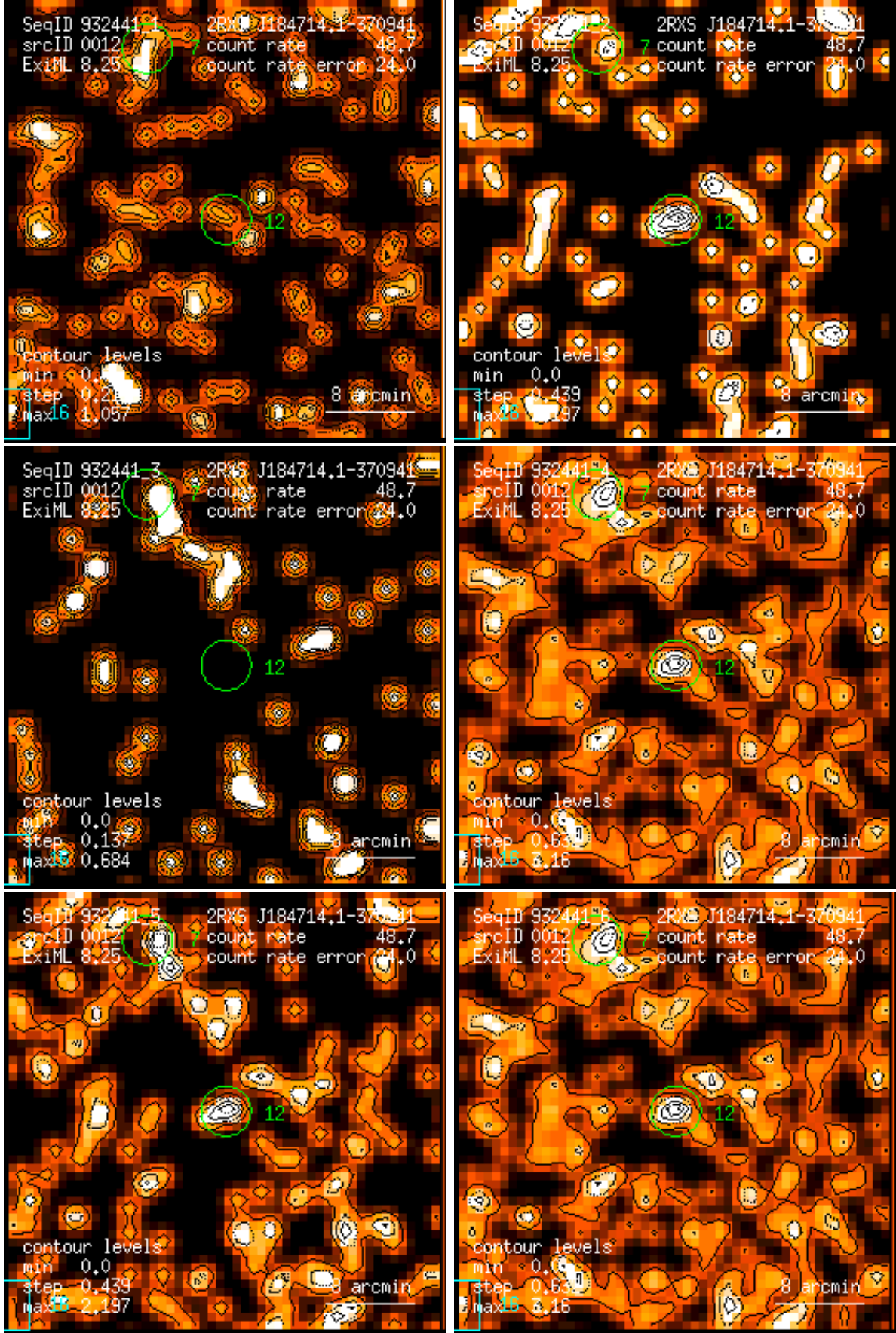
Figure 12: RASS 932441: detection 0012: band rate images, Gaussian filter: (1) PSPC channels 11 – 41, (2) 52 – 90, (3) 91 – 201, (4) 11 – 235, (5) 52 – 201, (6) 11 – 201. Broad band rates in counts/ks. Band rate contour levels in counts/ks/arcmin 2 .
