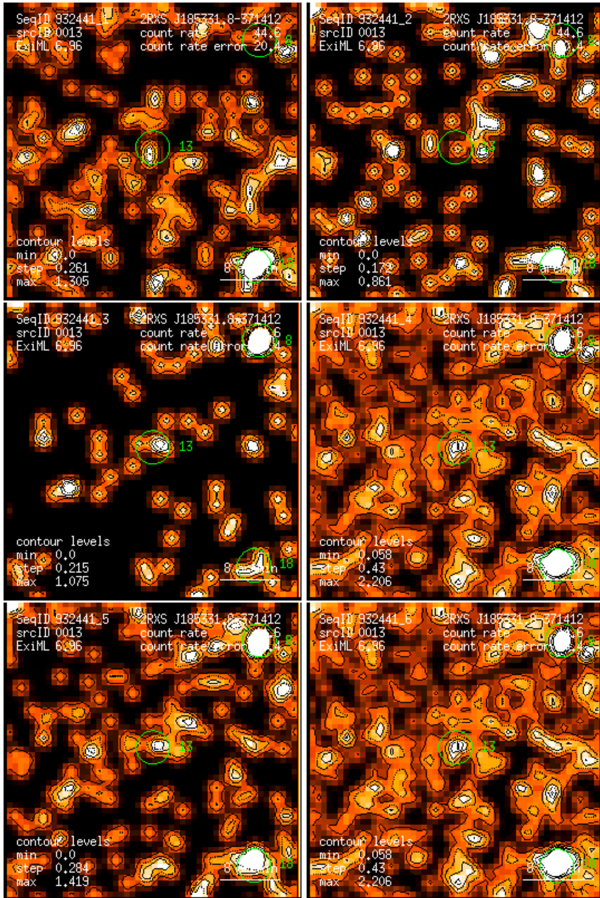
Figure 13: RASS 932441: detection 0013: band rate images, Gaussian filter: (1) PSPC channels 11 – 41, (2) 52 – 90, (3) 91 – 201, (4) 11 – 235, (5) 52 – 201, (6) 11 – 201. Broad band rates in counts/ks. Band rate contour levels in counts/ks/arcmin 2 .
