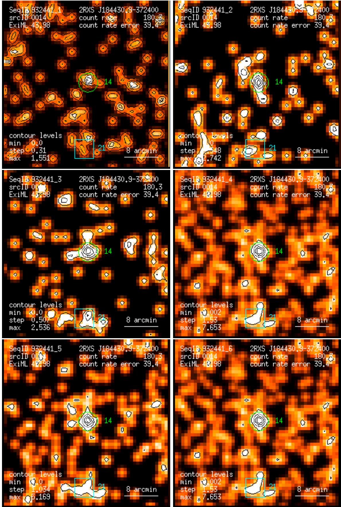
Figure 14: RASS 932441: detection 0014: band rate images, Gaussian filter: (1) PSPC channels 11 – 41, (2) 52 – 90, (3) 91 – 201, (4) 11 – 235, (5) 52 – 201, (6) 11 – 201. Broad band rates in counts/ks. Band rate contour levels in counts/ks/arcmin 2 .
