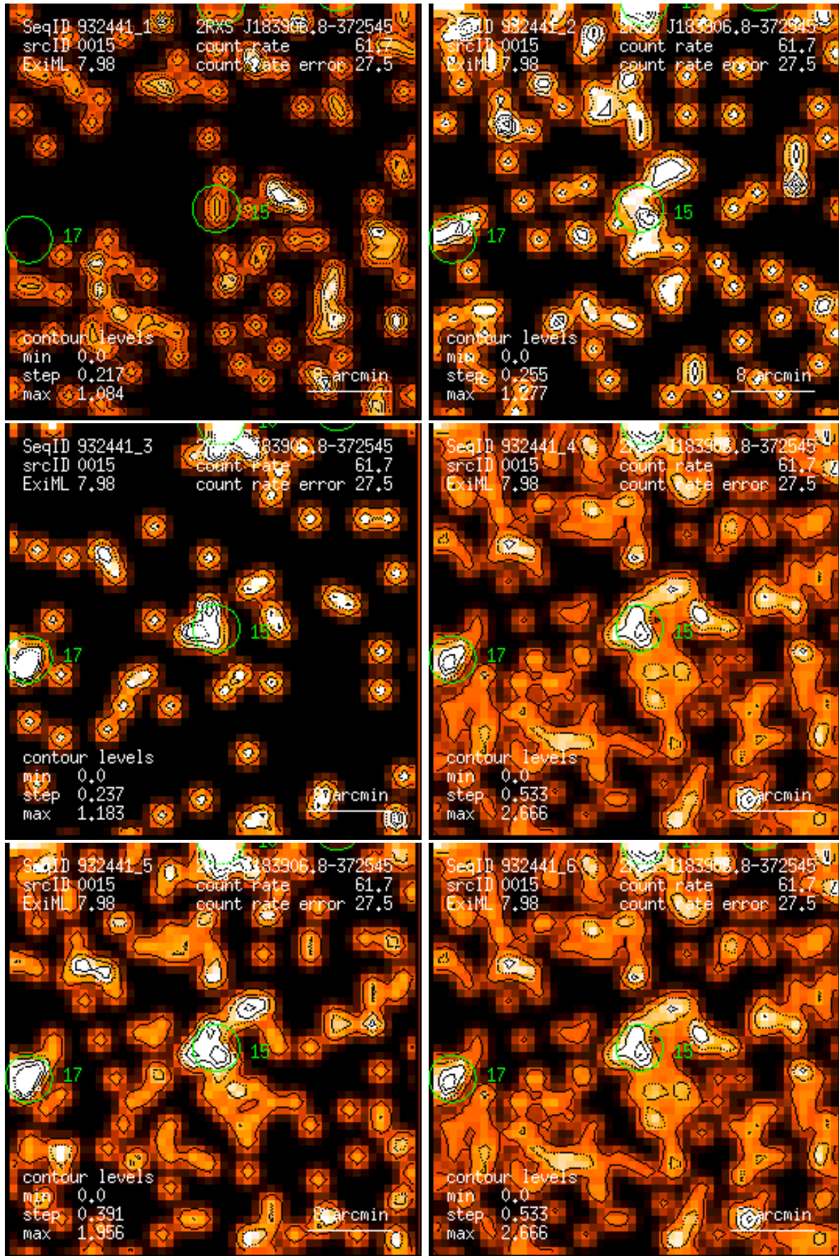
Figure 15: RASS 932441: detection 0015: band rate images, Gaussian filter: (1) PSPC channels 11 – 41, (2) 52 – 90, (3) 91 – 201, (4) 11 – 235, (5) 52 – 201, (6) 11 – 201. Broad band rates in counts/ks. Band rate contour levels in counts/ks/arcmin 2 .
