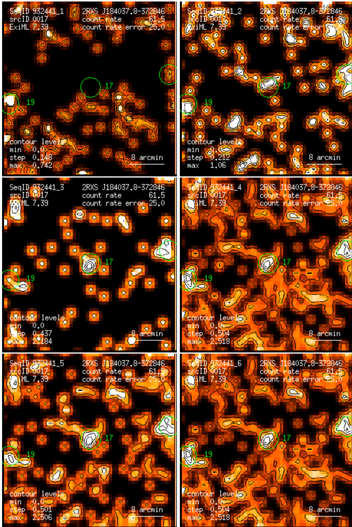
Figure 17: RASS 932441: detection 0017: band rate images, Gaussian filter: (1) PSPC channels 11 – 41, (2) 52 – 90, (3) 91 – 201, (4) 11 – 235, (5) 52 – 201, (6) 11 – 201. Broad band rates in counts/ks. Band rate contour levels in counts/ks/arcmin 2 .
