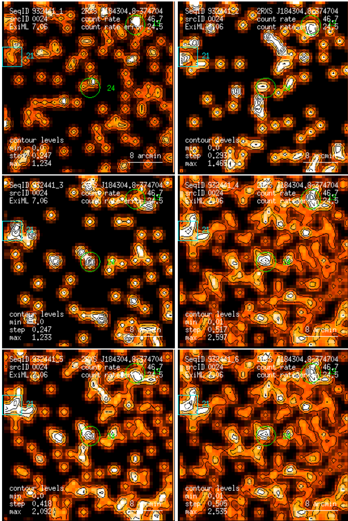
Figure 24: RASS 932441: detection 0024: band rate images, Gaussian filter: (1) PSPC channels 11 – 41, (2) 52 – 90, (3) 91 – 201, (4) 11 – 235, (5) 52 – 201, (6) 11 – 201. Broad band rates in counts/ks. Band rate contour levels in counts/ks/arcmin 2 .
