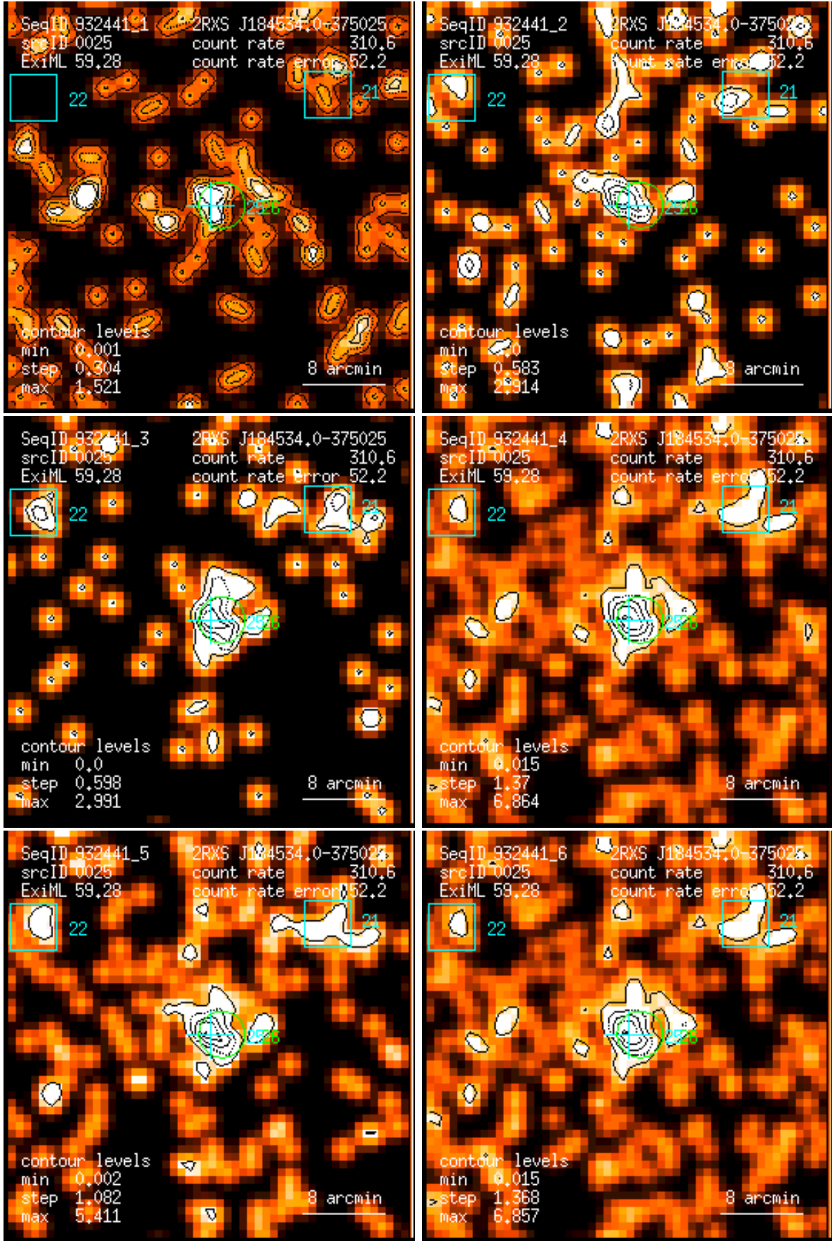
Figure 25: RASS 932441: detection 0025: band rate images, Gaussian filter: (1) PSPC channels 11 – 41, (2) 52 – 90, (3) 91 – 201, (4) 11 – 235, (5) 52 – 201, (6) 11 – 201. Broad band rates in counts/ks. Band rate contour levels in counts/ks/arcmin 2 .
