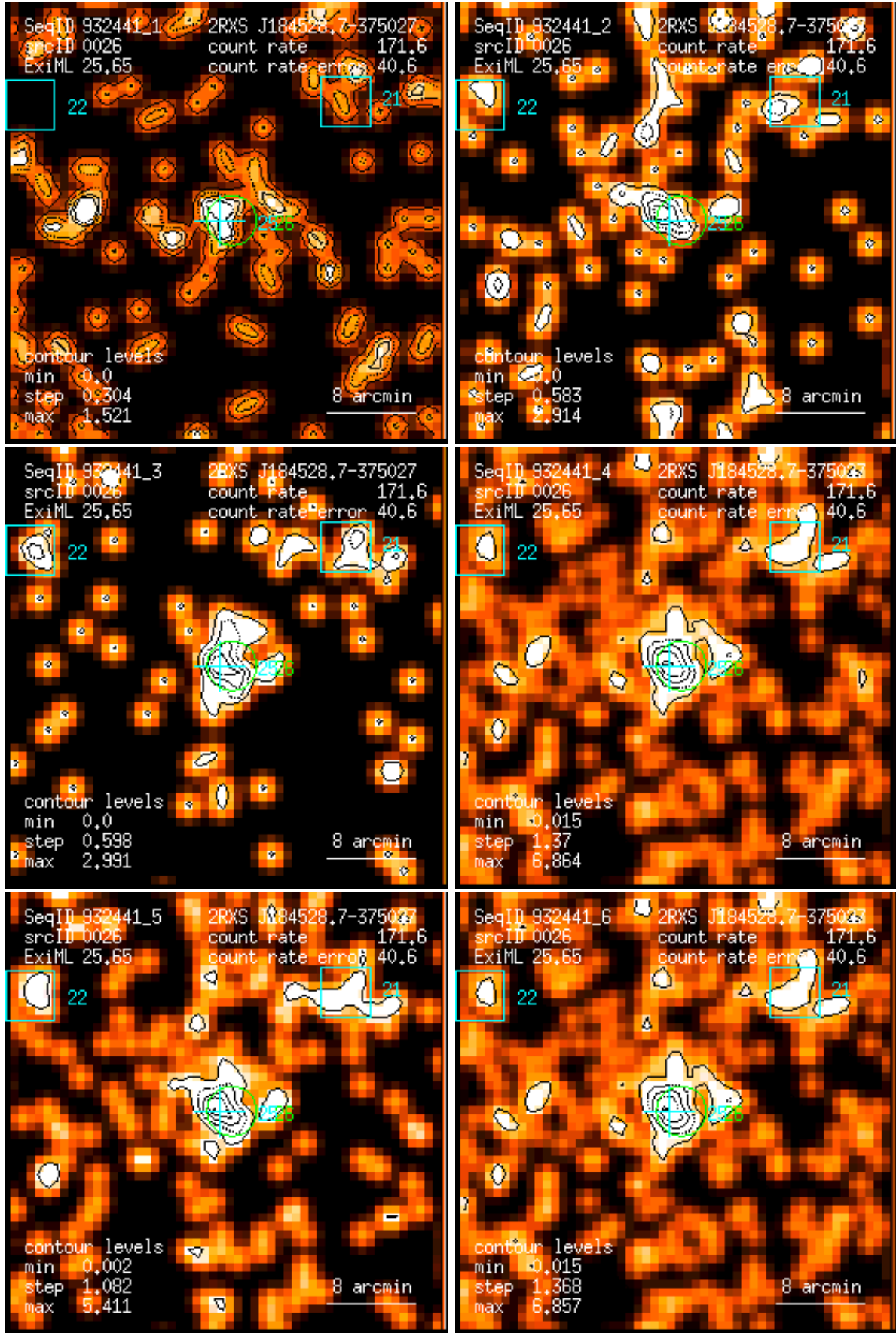
Figure 26: RASS 932441: detection 0026: band rate images, Gaussian filter: (1) PSPC channels 11 – 41, (2) 52 – 90, (3) 91 – 201, (4) 11 – 235, (5) 52 – 201, (6) 11 – 201. Broad band rates in counts/ks. Band rate contour levels in counts/ks/arcmin 2 .
