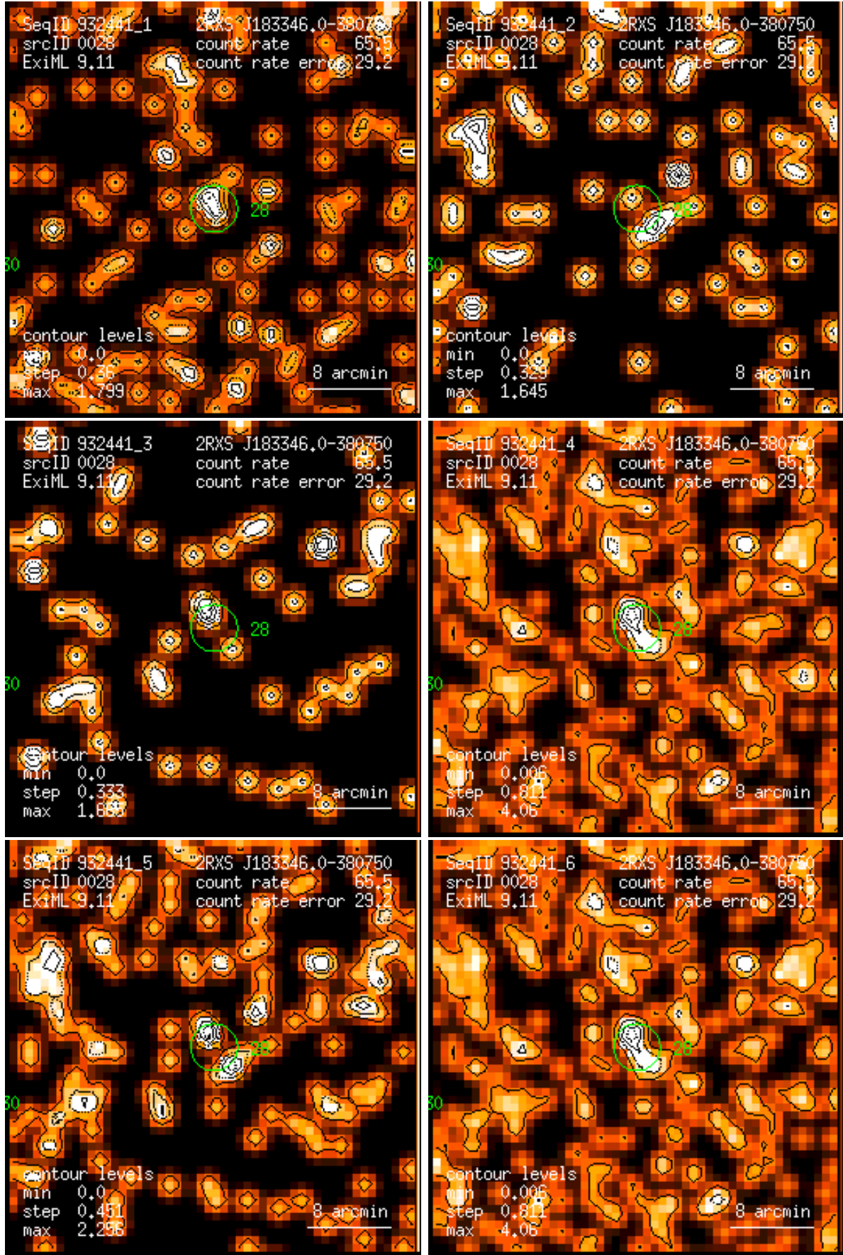
Figure 28: RASS 932441: detection 0028: band rate images, Gaussian filter: (1) PSPC channels 11 – 41, (2) 52 – 90, (3) 91 – 201, (4) 11 – 235, (5) 52 – 201, (6) 11 – 201. Broad band rates in counts/ks. Band rate contour levels in counts/ks/arcmin 2 .
