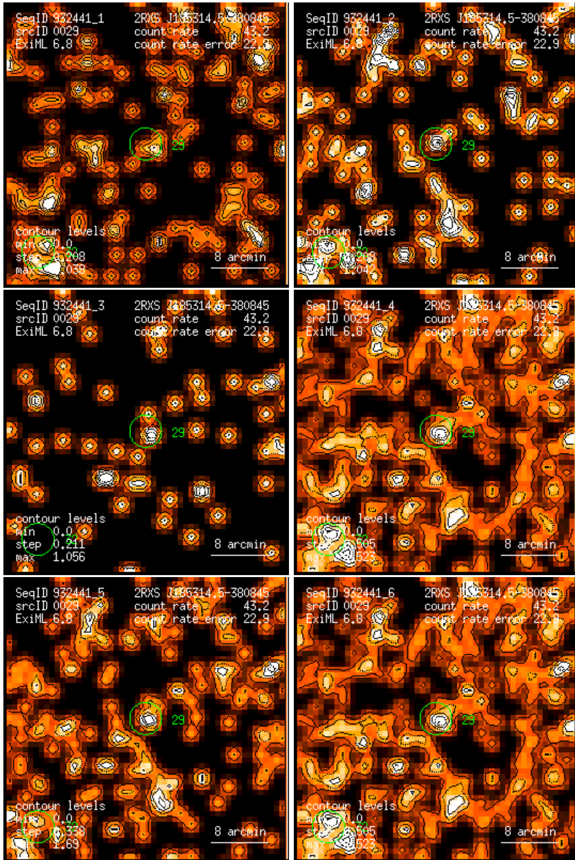
Figure 29: RASS 932441: detection 0029: band rate images, Gaussian filter: (1) PSPC channels 11 – 41, (2) 52 – 90, (3) 91 – 201, (4) 11 – 235, (5) 52 – 201, (6) 11 – 201. Broad band rates in counts/ks. Band rate contour levels in counts/ks/arcmin 2 .
