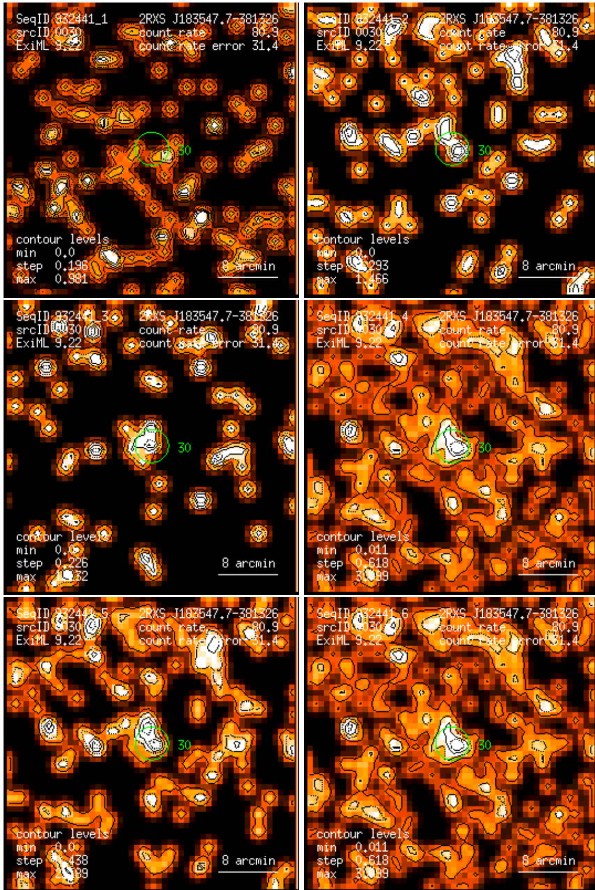
Figure 30: RASS 932441: detection 0030: band rate images, Gaussian filter: (1) PSPC channels 11 – 41, (2) 52 – 90, (3) 91 – 201, (4) 11 – 235, (5) 52 – 201, (6) 11 – 201. Broad band rates in counts/ks. Band rate contour levels in counts/ks/arcmin 2 .
