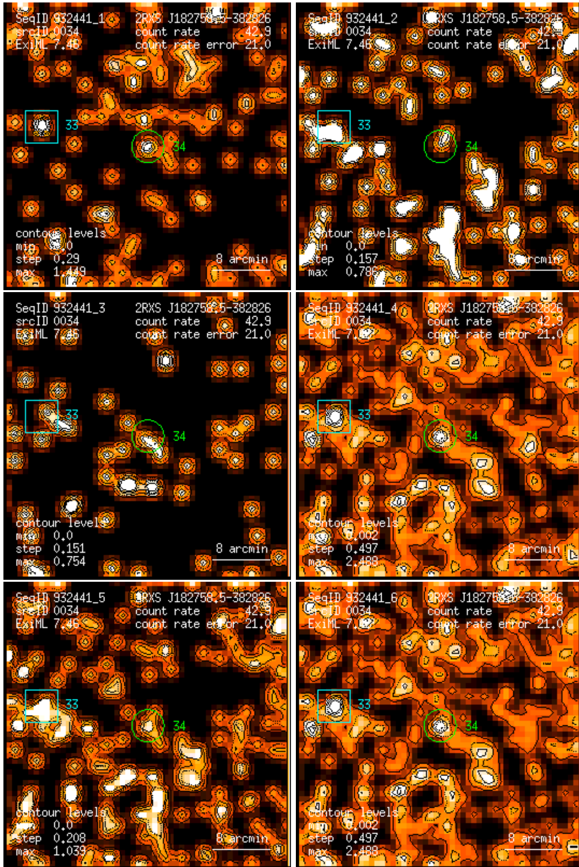
Figure 34: RASS 932441: detection 0034: band rate images, Gaussian filter: (1) PSPC channels 11 – 41, (2) 52 – 90, (3) 91 – 201, (4) 11 – 235, (5) 52 – 201, (6) 11 – 201. Broad band rates in counts/ks. Band rate contour levels in counts/ks/arcmin 2 .
