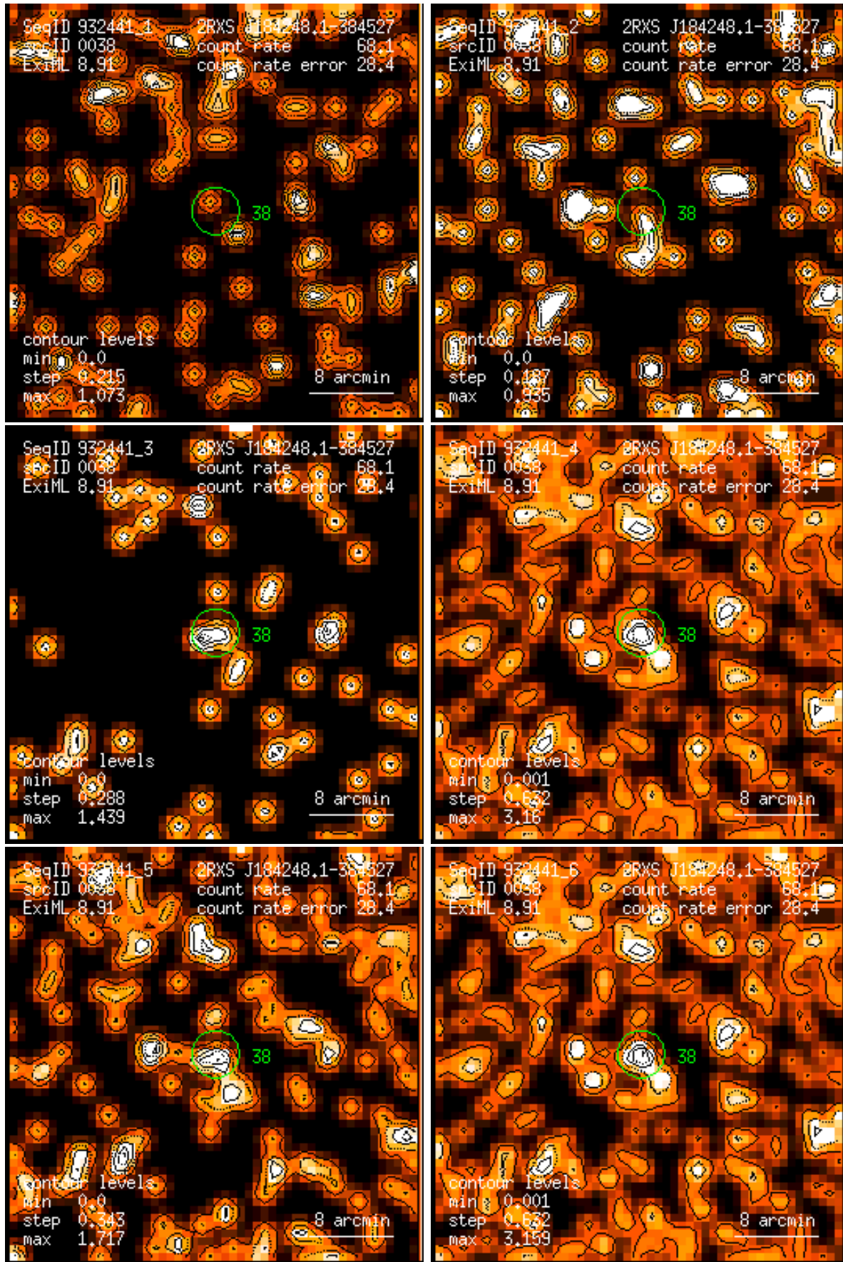
Figure 38: RASS 932441: detection 0038: band rate images, Gaussian filter: (1) PSPC channels 11 – 41, (2) 52 – 90, (3) 91 – 201, (4) 11 – 235, (5) 52 – 201, (6) 11 – 201. Broad band rates in counts/ks. Band rate contour levels in counts/ks/arcmin 2 .
