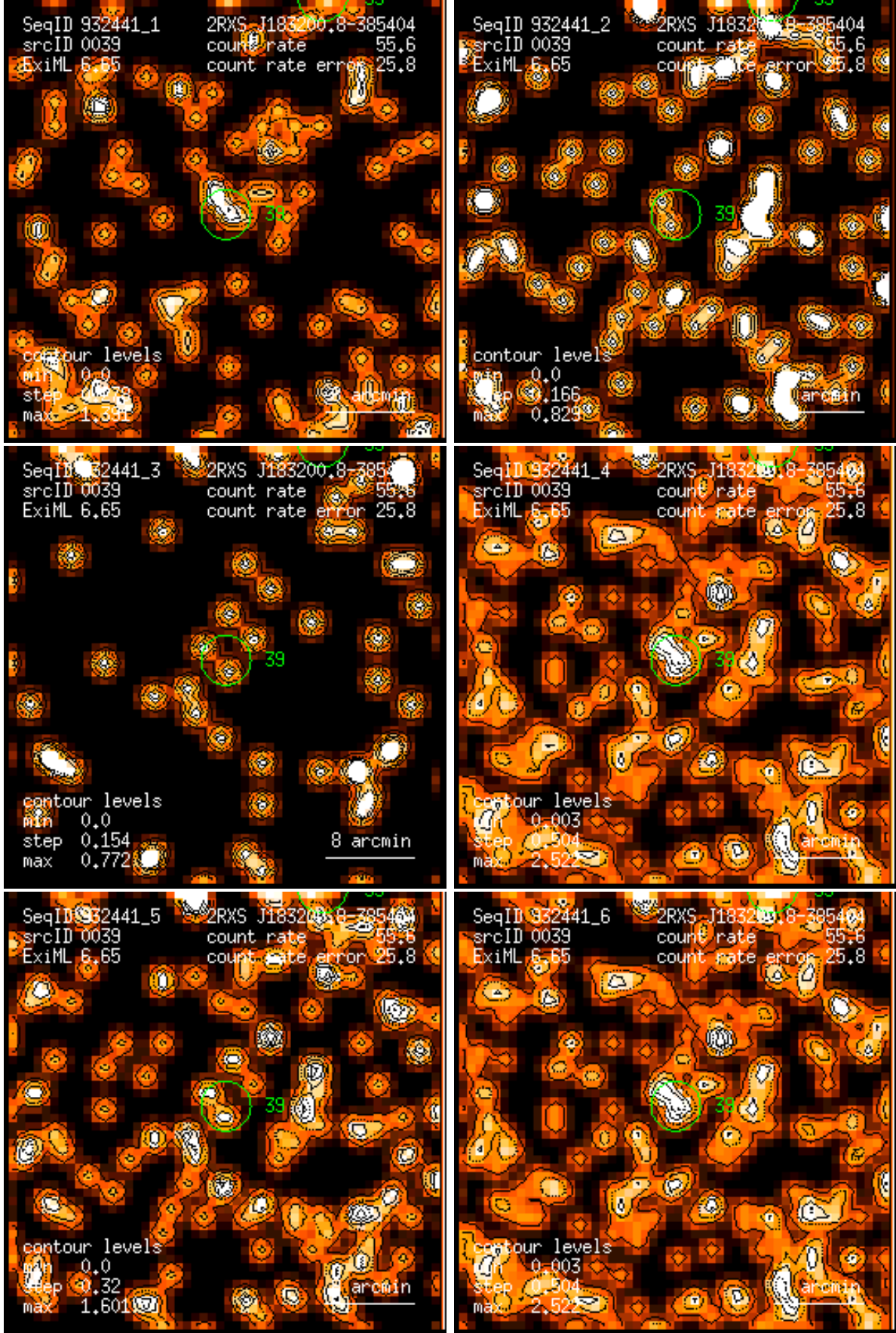
Figure 39: RASS 932441: detection 0039: band rate images, Gaussian filter: (1) PSPC channels 11 – 41, (2) 52 – 90, (3) 91 – 201, (4) 11 – 235, (5) 52 – 201, (6) 11 – 201. Broad band rates in counts/ks. Band rate contour levels in counts/ks/arcmin 2 .
