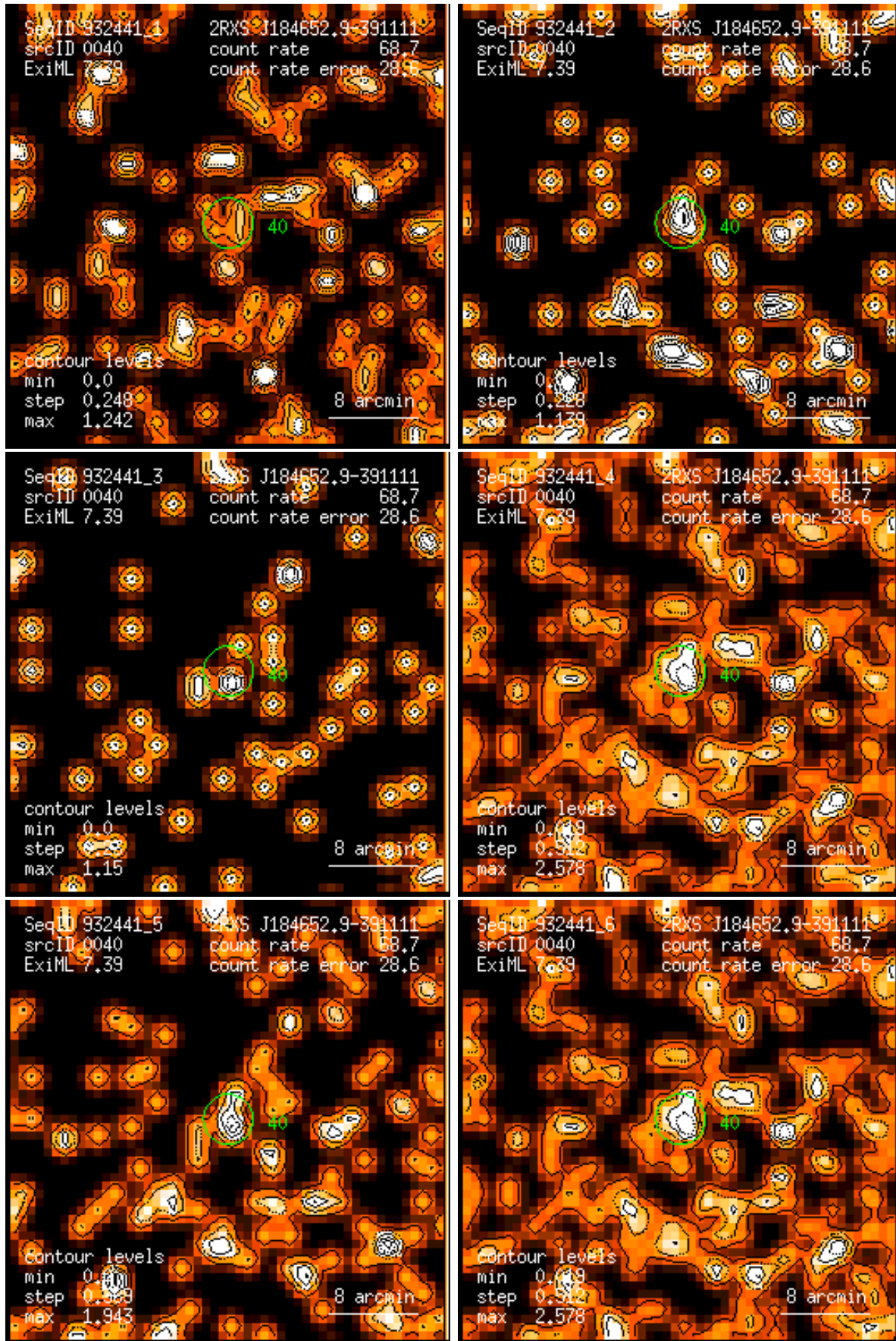
Figure 40: RASS 932441: detection 0040: band rate images, Gaussian filter: (1) PSPC channels 11 – 41, (2) 52 – 90, (3) 91 – 201, (4) 11 – 235, (5) 52 – 201, (6) 11 – 201. Broad band rates in counts/ks. Band rate contour levels in counts/ks/arcmin 2 .
