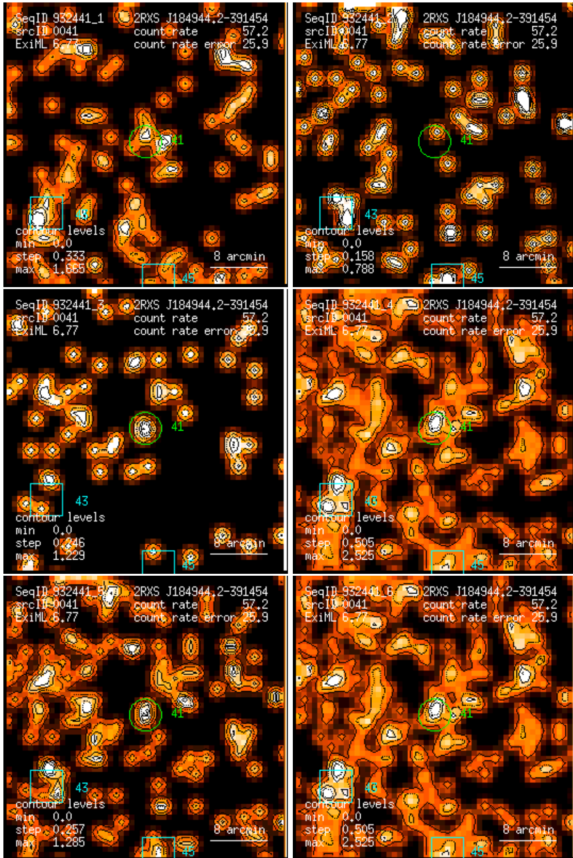
Figure 41: RASS 932441: detection 0041: band rate images, Gaussian filter: (1) PSPC channels 11 – 41, (2) 52 – 90, (3) 91 – 201, (4) 11 – 235, (5) 52 – 201, (6) 11 – 201. Broad band rates in counts/ks. Band rate contour levels in counts/ks/arcmin 2 .
