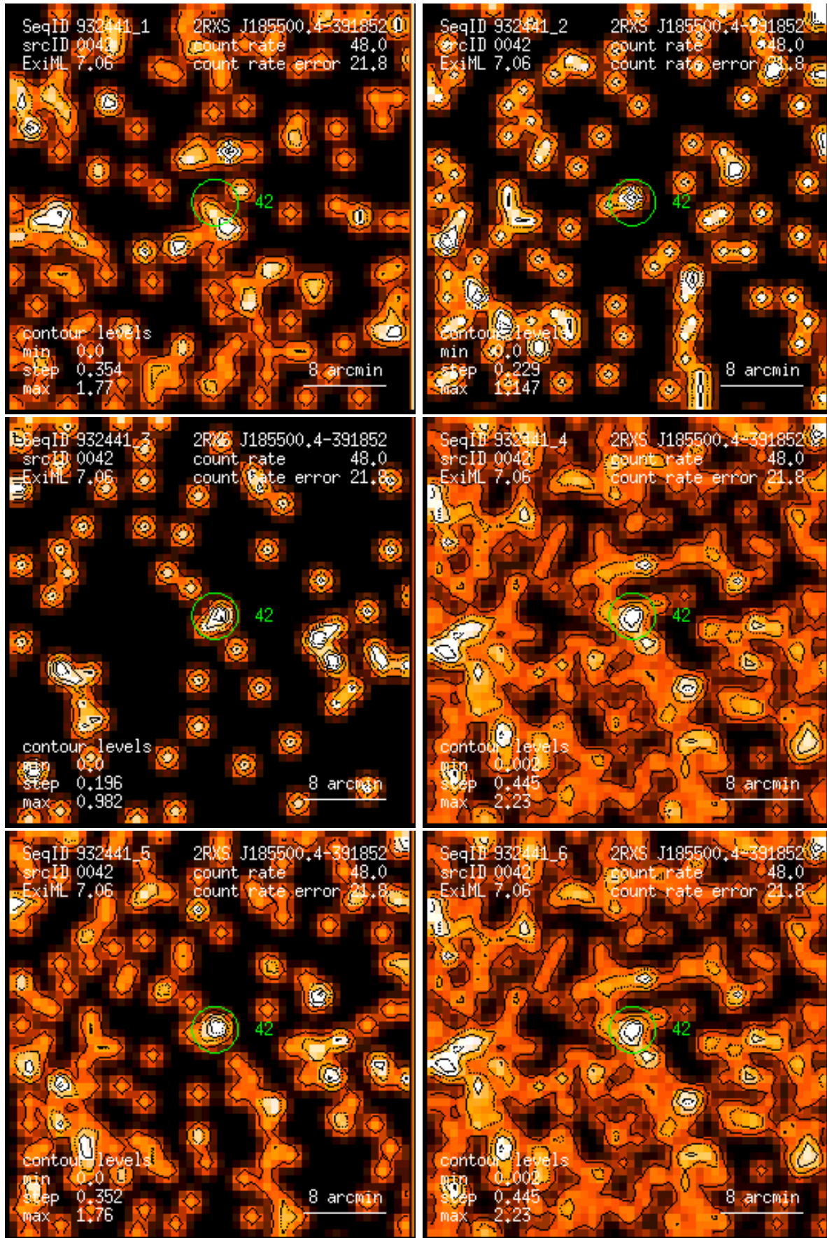
Figure 42: RASS 932441: detection 0042: band rate images, Gaussian filter: (1) PSPC channels 11 – 41, (2) 52 – 90, (3) 91 – 201, (4) 11 – 235, (5) 52 – 201, (6) 11 – 201. Broad band rates in counts/ks. Band rate contour levels in counts/ks/arcmin 2 .
