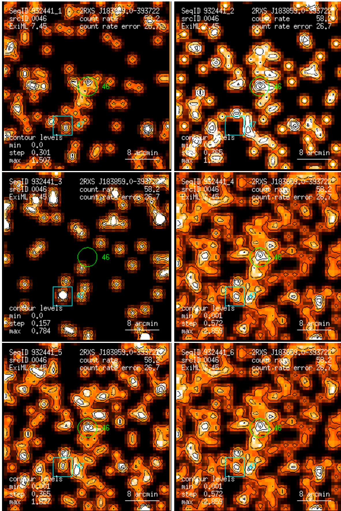
Figure 46: RASS 932441: detection 0046: band rate images, Gaussian filter: (1) PSPC channels 11 – 41, (2) 52 – 90, (3) 91 – 201, (4) 11 – 235, (5) 52 – 201, (6) 11 – 201. Broad band rates in counts/ks. Band rate contour levels in counts/ks/arcmin 2 .
