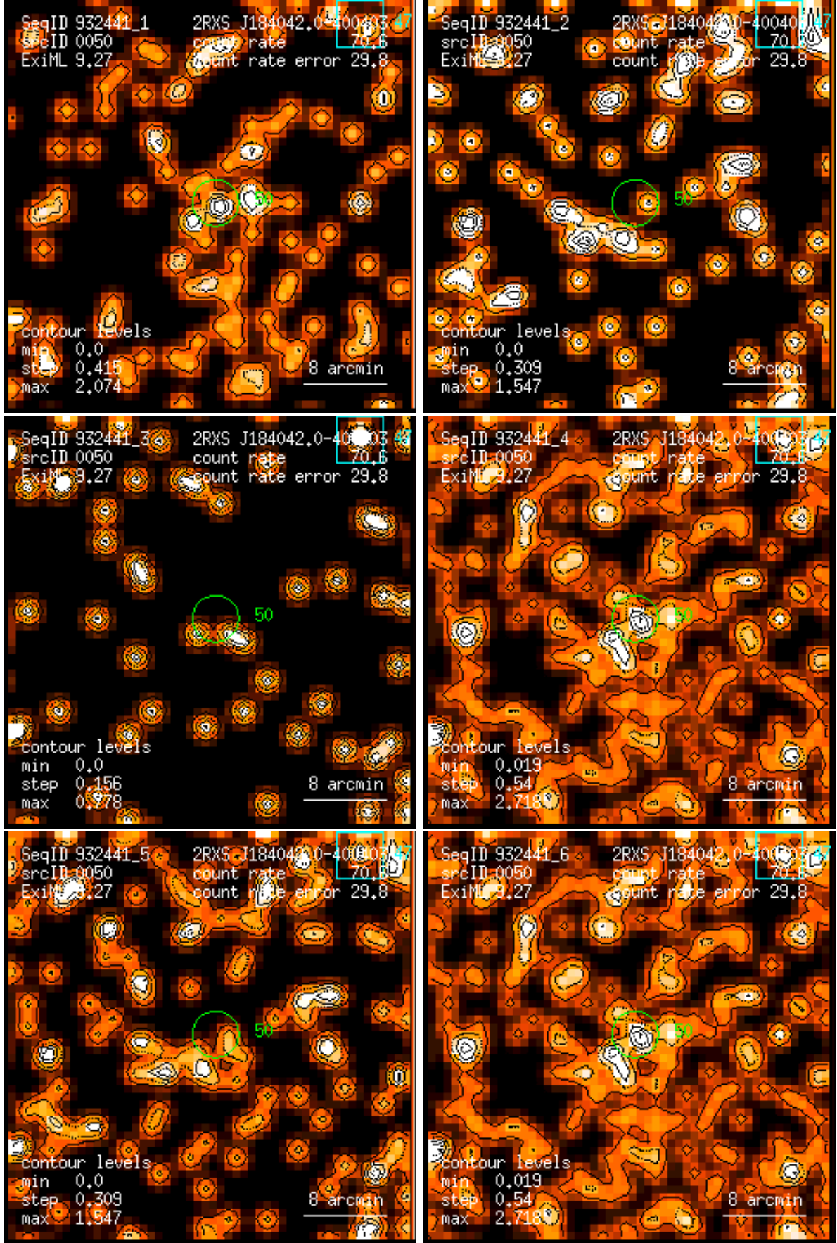
Figure 50: RASS 932441: detection 0050: band rate images, Gaussian filter: (1) PSPC channels 11 – 41, (2) 52 – 90, (3) 91 – 201, (4) 11 – 235, (5) 52 – 201, (6) 11 – 201. Broad band rates in counts/ks. Band rate contour levels in counts/ks/arcmin 2 .
