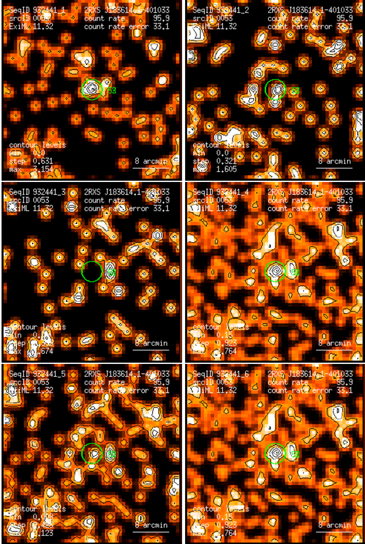
Figure 53: RASS 932441: detection 0053: band rate images, Gaussian filter: (1) PSPC channels 11 – 41, (2) 52 – 90, (3) 91 – 201, (4) 11 – 235, (5) 52 – 201, (6) 11 – 201. Broad band rates in counts/ks. Band rate contour levels in counts/ks/arcmin 2 .
