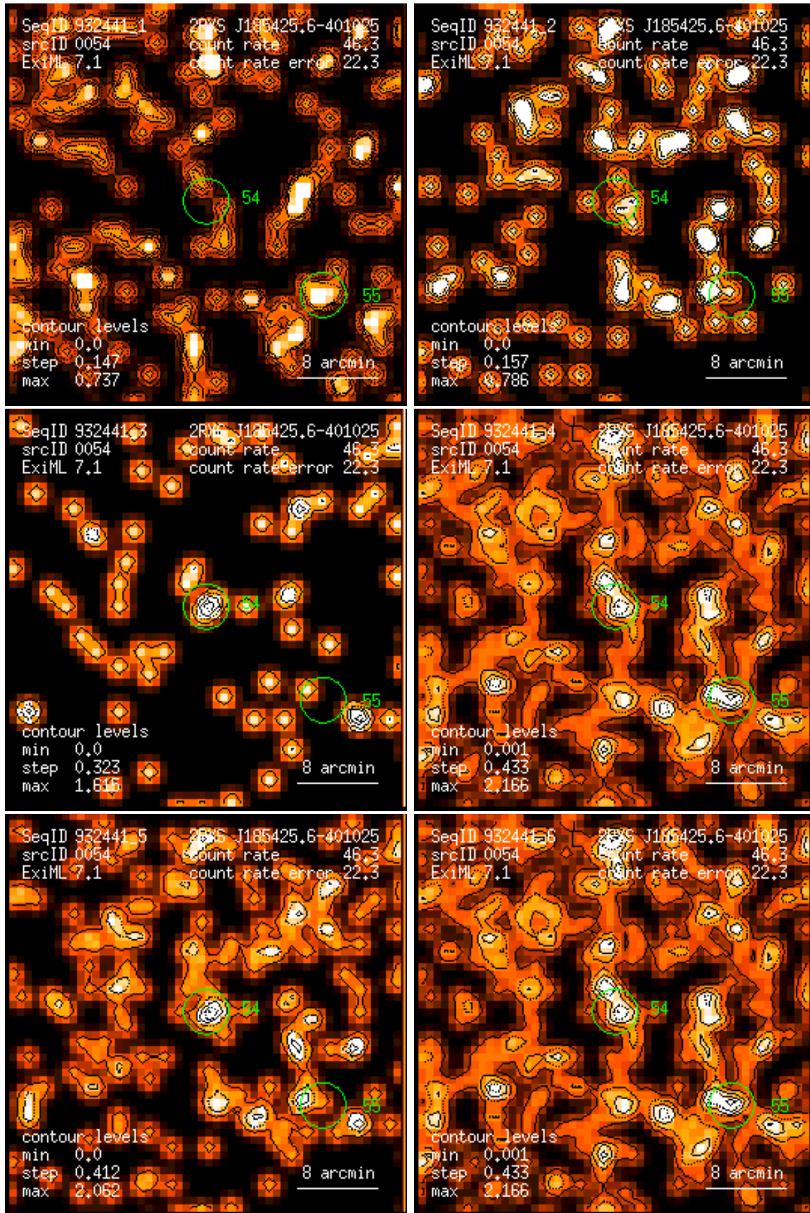
Figure 54: RASS 932441: detection 0054: band rate images, Gaussian filter: (1) PSPC channels 11 – 41, (2) 52 – 90, (3) 91 – 201, (4) 11 – 235, (5) 52 – 201, (6) 11 – 201. Broad band rates in counts/ks. Band rate contour levels in counts/ks/arcmin 2 .
