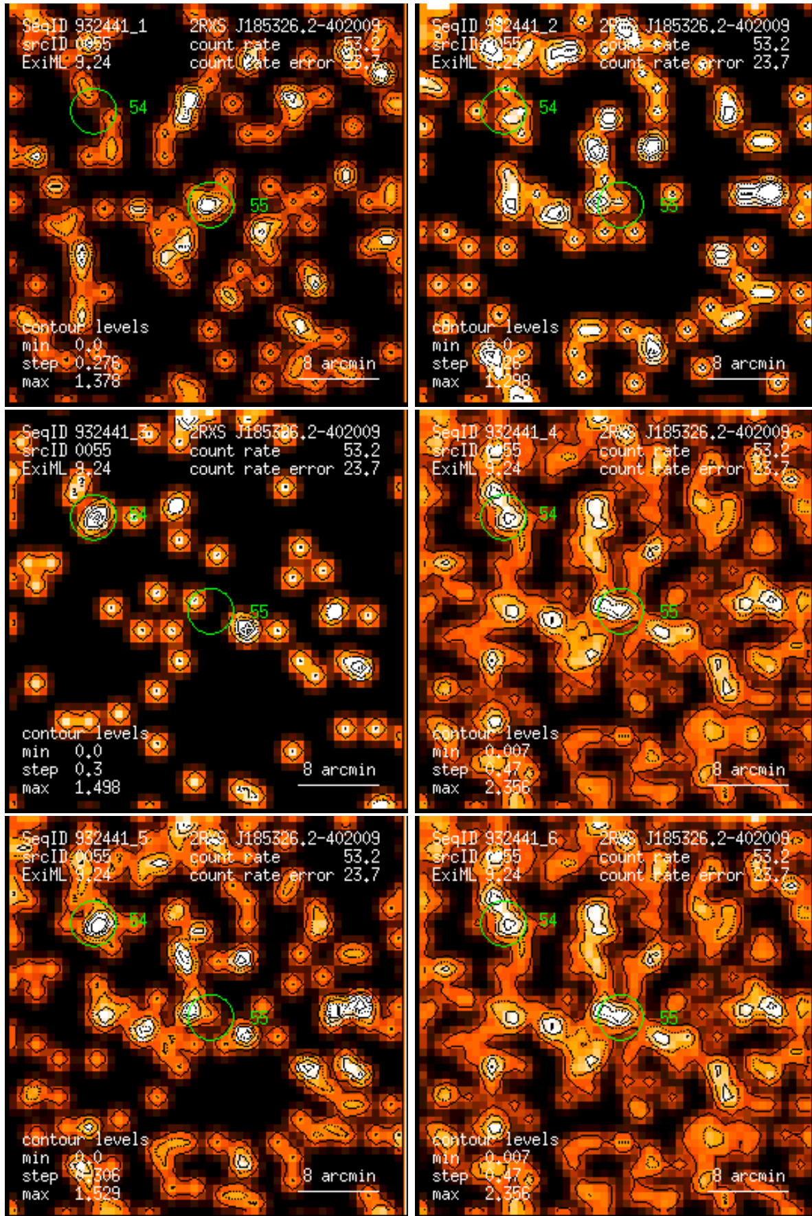
Figure 55: RASS 932441: detection 0055: band rate images, Gaussian filter: (1) PSPC channels 11 – 41, (2) 52 – 90, (3) 91 – 201, (4) 11 – 235, (5) 52 – 201, (6) 11 – 201. Broad band rates in counts/ks. Band rate contour levels in counts/ks/arcmin 2 .
