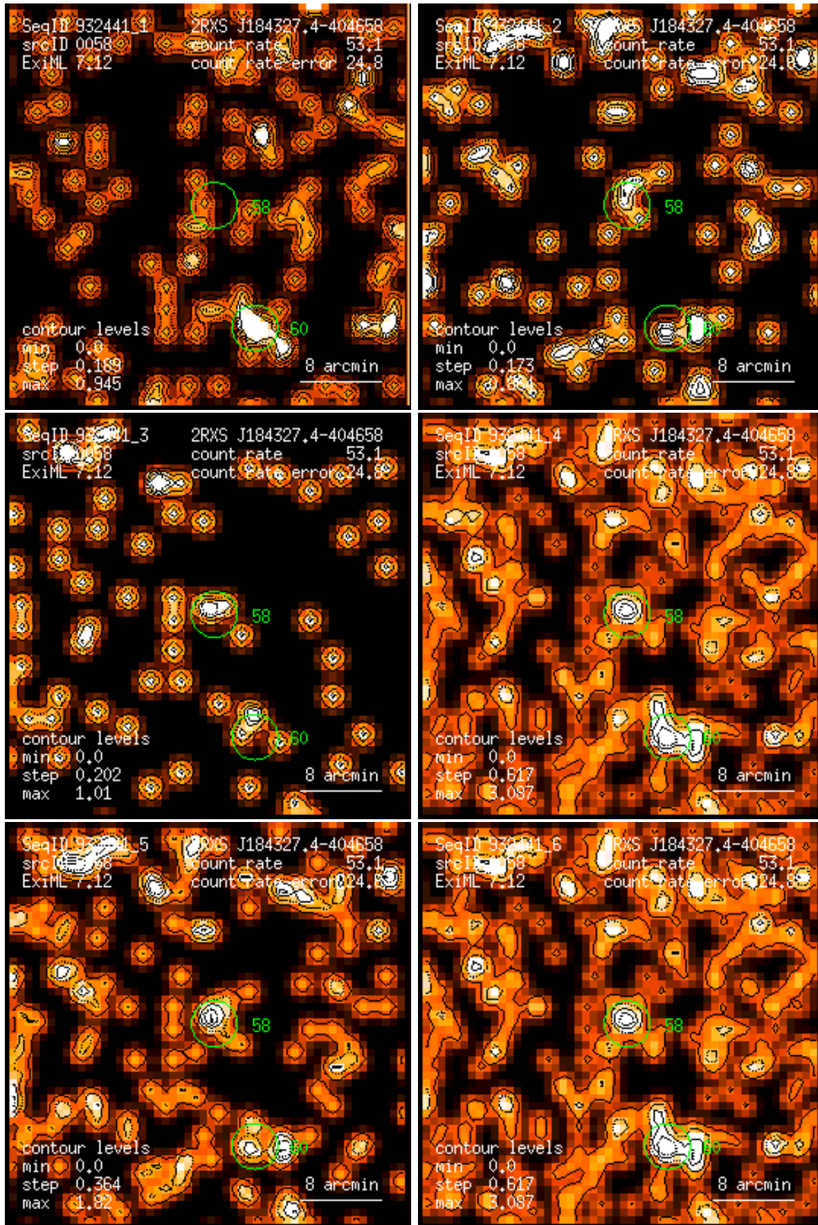
Figure 58: RASS 932441: detection 0058: band rate images, Gaussian filter: (1) PSPC channels 11 – 41, (2) 52 – 90, (3) 91 – 201, (4) 11 – 235, (5) 52 – 201, (6) 11 – 201. Broad band rates in counts/ks. Band rate contour levels in counts/ks/arcmin 2 .
