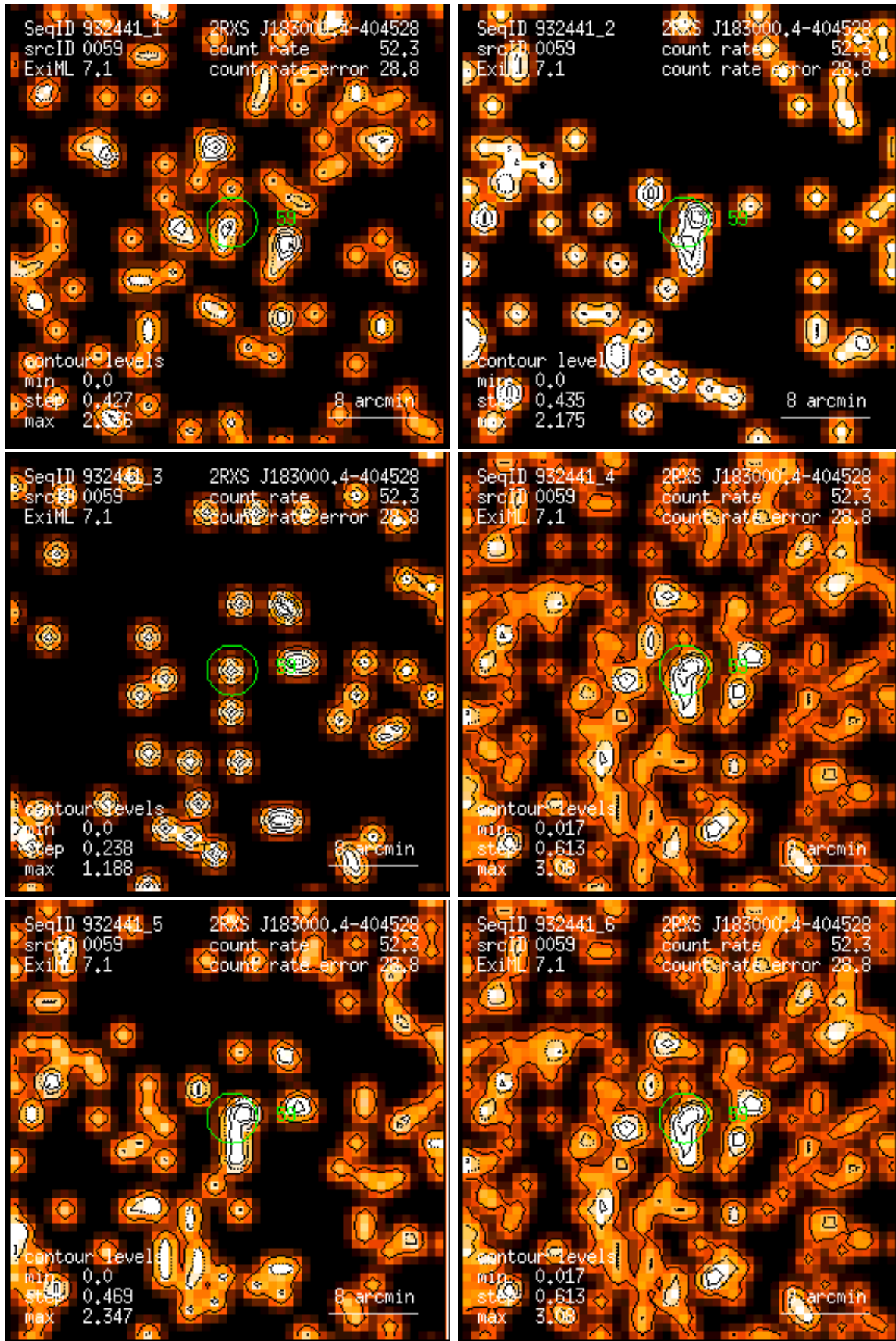
Figure 59: RASS 932441: detection 0059: band rate images, Gaussian filter: (1) PSPC channels 11 – 41, (2) 52 – 90, (3) 91 – 201, (4) 11 – 235, (5) 52 – 201, (6) 11 – 201. Broad band rates in counts/ks. Band rate contour levels in counts/ks/arcmin 2 .
