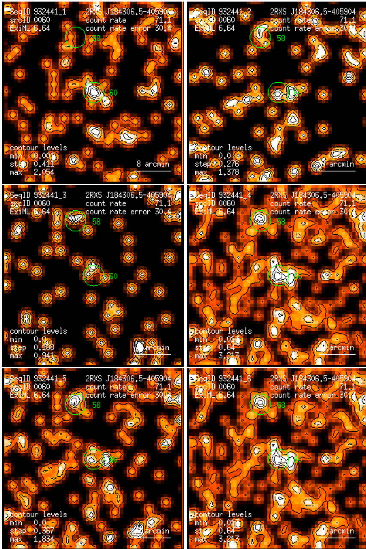
Figure 60: RASS 932441: detection 0060: band rate images, Gaussian filter: (1) PSPC channels 11 – 41, (2) 52 – 90, (3) 91 – 201, (4) 11 – 235, (5) 52 – 201, (6) 11 – 201. Broad band rates in counts/ks. Band rate contour levels in counts/ks/arcmin 2 .
