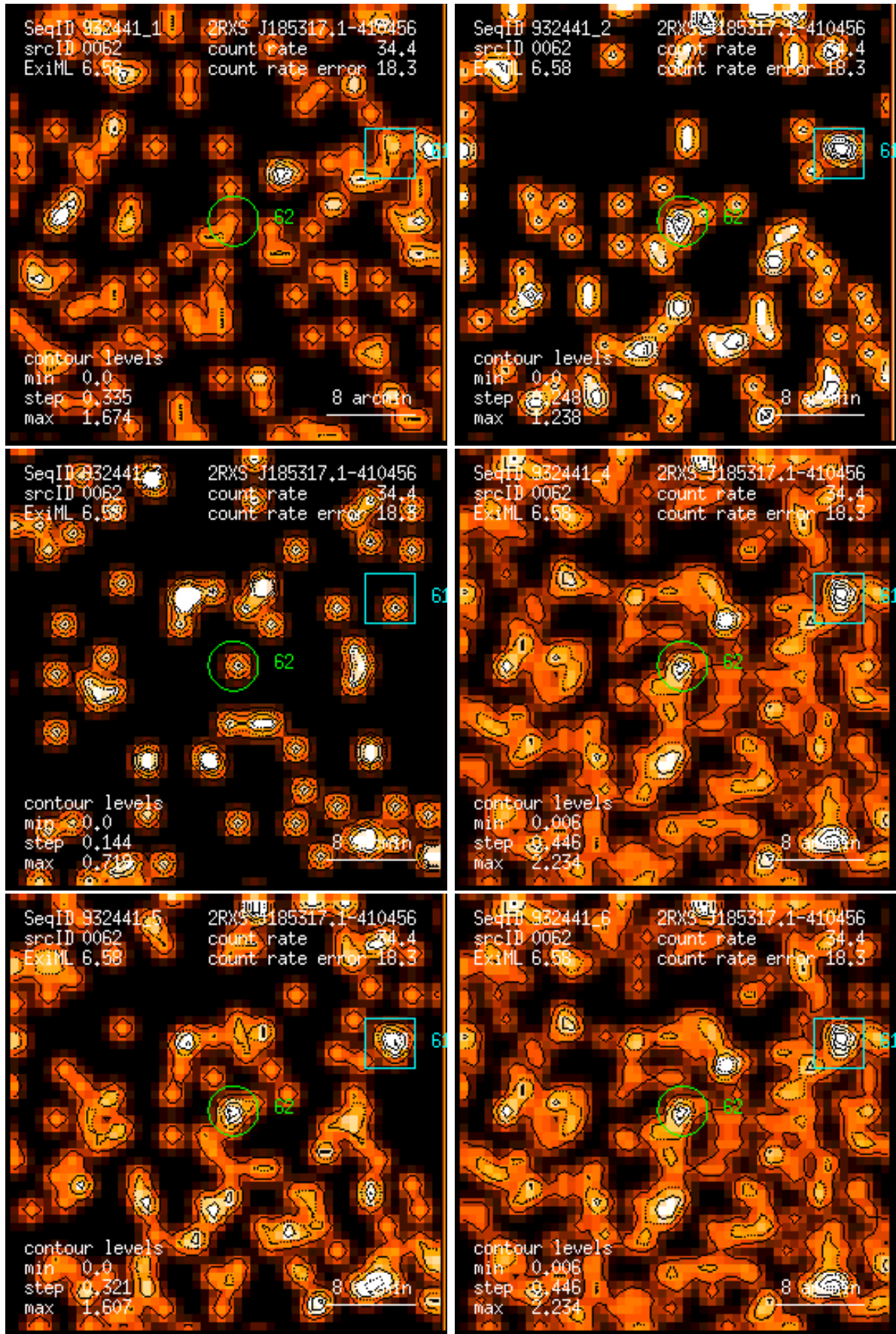
Figure 62: RASS 932441: detection 0062: band rate images, Gaussian filter: (1) PSPC channels 11 – 41, (2) 52 – 90, (3) 91 – 201, (4) 11 – 235, (5) 52 – 201, (6) 11 – 201. Broad band rates in counts/ks. Band rate contour levels in counts/ks/arcmin 2 .
