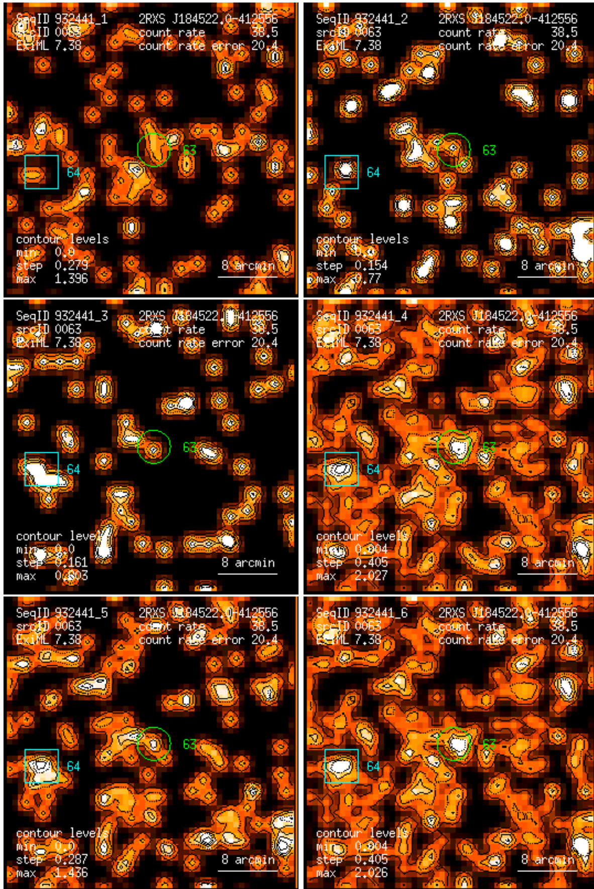
Figure 63: RASS 932441: detection 0063: band rate images, Gaussian filter: (1) PSPC channels 11 – 41, (2) 52 – 90, (3) 91 – 201, (4) 11 – 235, (5) 52 – 201, (6) 11 – 201. Broad band rates in counts/ks. Band rate contour levels in counts/ks/arcmin 2 .
