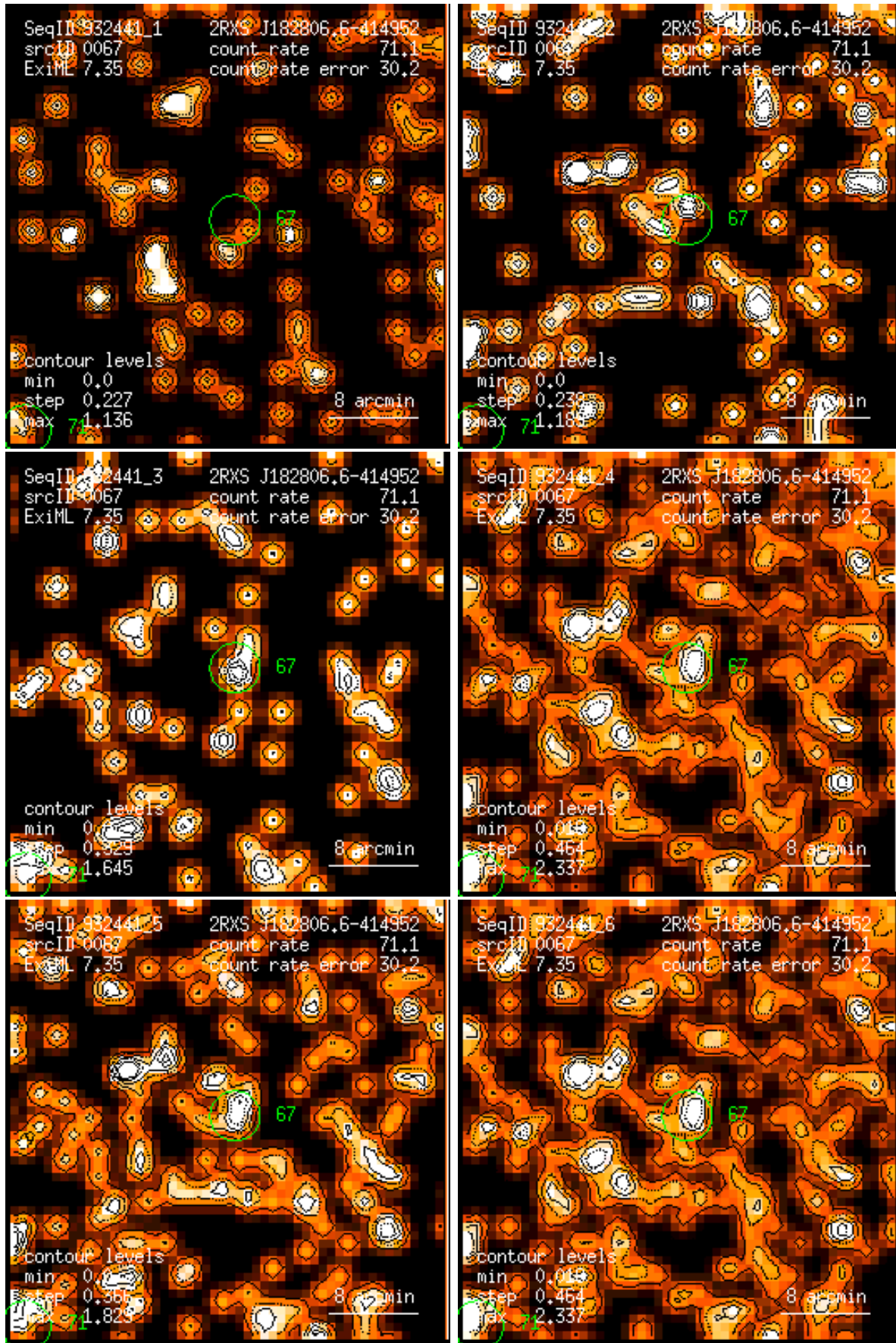
Figure 67: RASS 932441: detection 0067: band rate images, Gaussian filter: (1) PSPC channels 11 – 41, (2) 52 – 90, (3) 91 – 201, (4) 11 – 235, (5) 52 – 201, (6) 11 – 201. Broad band rates in counts/ks. Band rate contour levels in counts/ks/arcmin 2 .
