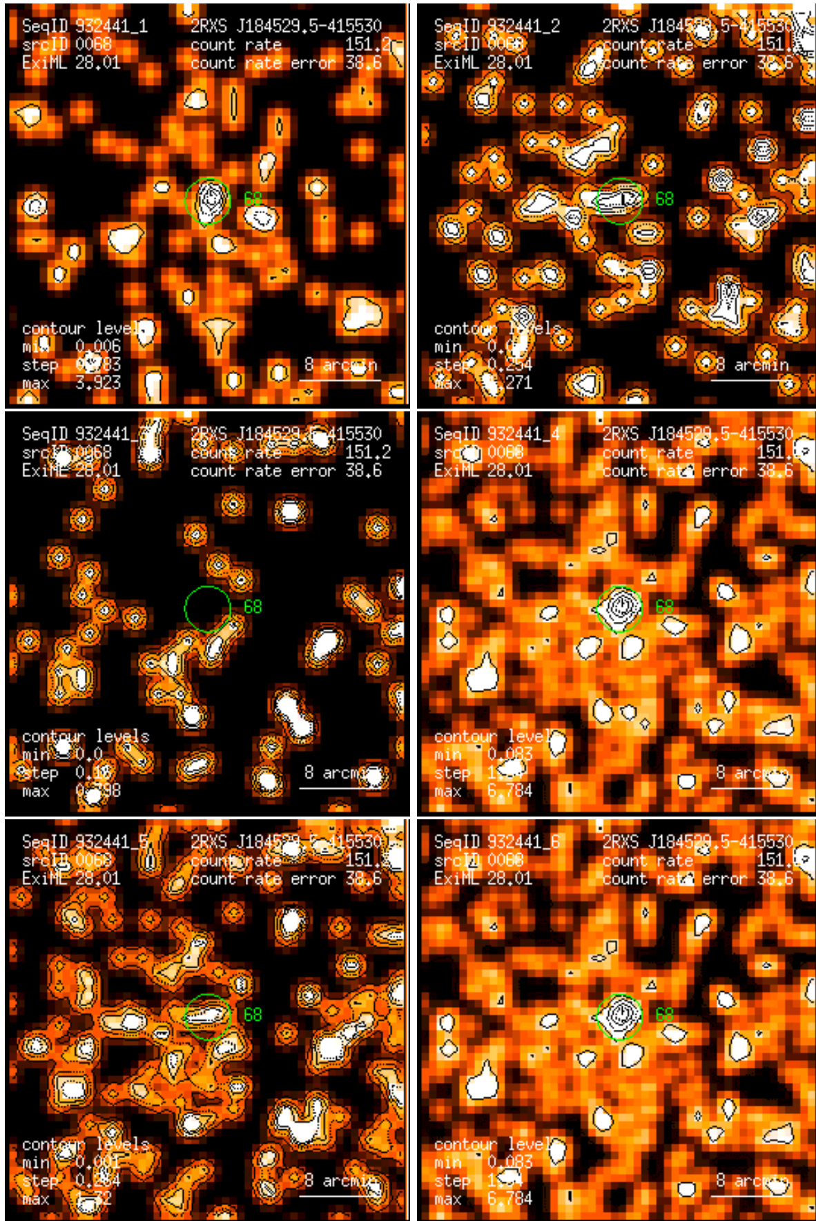
Figure 68: RASS 932441: detection 0068: band rate images, Gaussian filter: (1) PSPC channels 11 – 41, (2) 52 – 90, (3) 91 – 201, (4) 11 – 235, (5) 52 – 201, (6) 11 – 201. Broad band rates in counts/ks. Band rate contour levels in counts/ks/arcmin 2 .
