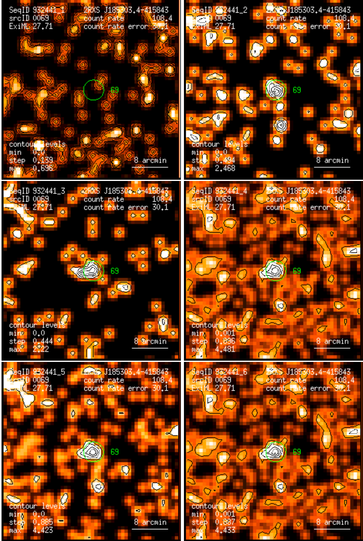
Figure 69: RASS 932441: detection 0069: band rate images, Gaussian filter: (1) PSPC channels 11 – 41, (2) 52 – 90, (3) 91 – 201, (4) 11 – 235, (5) 52 – 201, (6) 11 – 201. Broad band rates in counts/ks. Band rate contour levels in counts/ks/arcmin 2 .
