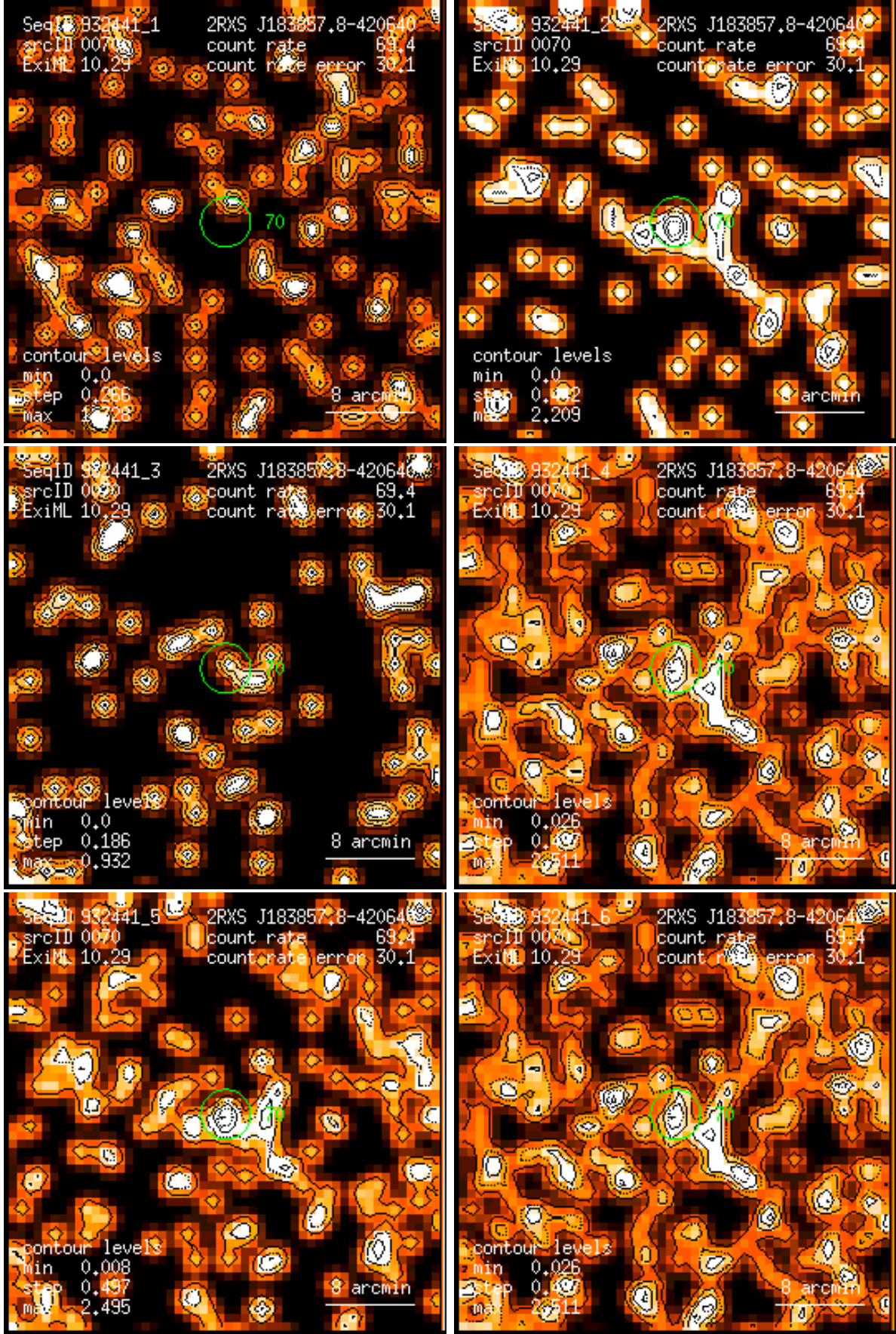
Figure 70: RASS 932441: detection 0070: band rate images, Gaussian filter: (1) PSPC channels 11 – 41, (2) 52 – 90, (3) 91 – 201, (4) 11 – 235, (5) 52 – 201, (6) 11 – 201. Broad band rates in counts/ks. Band rate contour levels in counts/ks/arcmin 2 .
