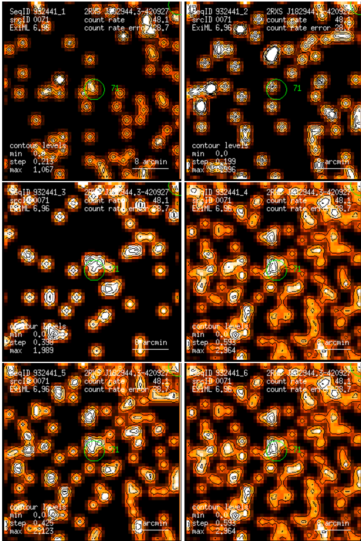
Figure 71: RASS 932441: detection 0071: band rate images, Gaussian filter: (1) PSPC channels 11 – 41, (2) 52 – 90, (3) 91 – 201, (4) 11 – 235, (5) 52 – 201, (6) 11 – 201. Broad band rates in counts/ks. Band rate contour levels in counts/ks/arcmin 2 .
