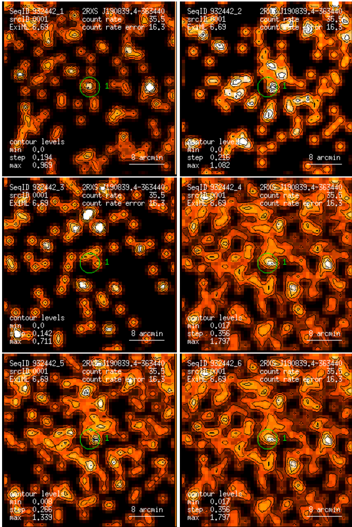
Figure 1: RASS 932442: detection 0001: band rate images, Gaussian filter: (1) PSPC channels 11 – 41, (2) 52 – 90, (3) 91 – 201, (4) 11 – 235, (5) 52 – 201, (6) 11 – 201. Broad band rates in counts/ks. Band rate contour levels in counts/ks/arcmin 2 .
